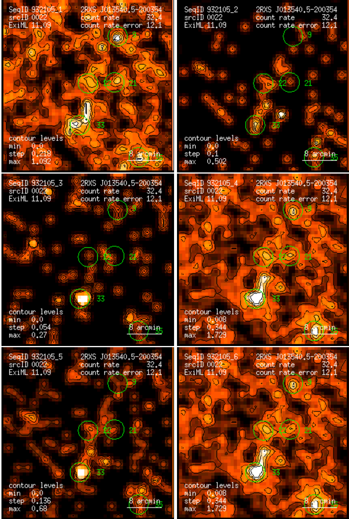
Figure 22: RASS 932105: detection 0022: band rate images, Gaussian filter: (1) PSPC channels 11 – 41, (2) 52 – 90, (3) 91 – 201, (4) 11 – 235, (5) 52 – 201, (6) 11 – 201. Broad band rates in counts/ks. Band rate contour levels in counts/ks/arcmin 2 .
