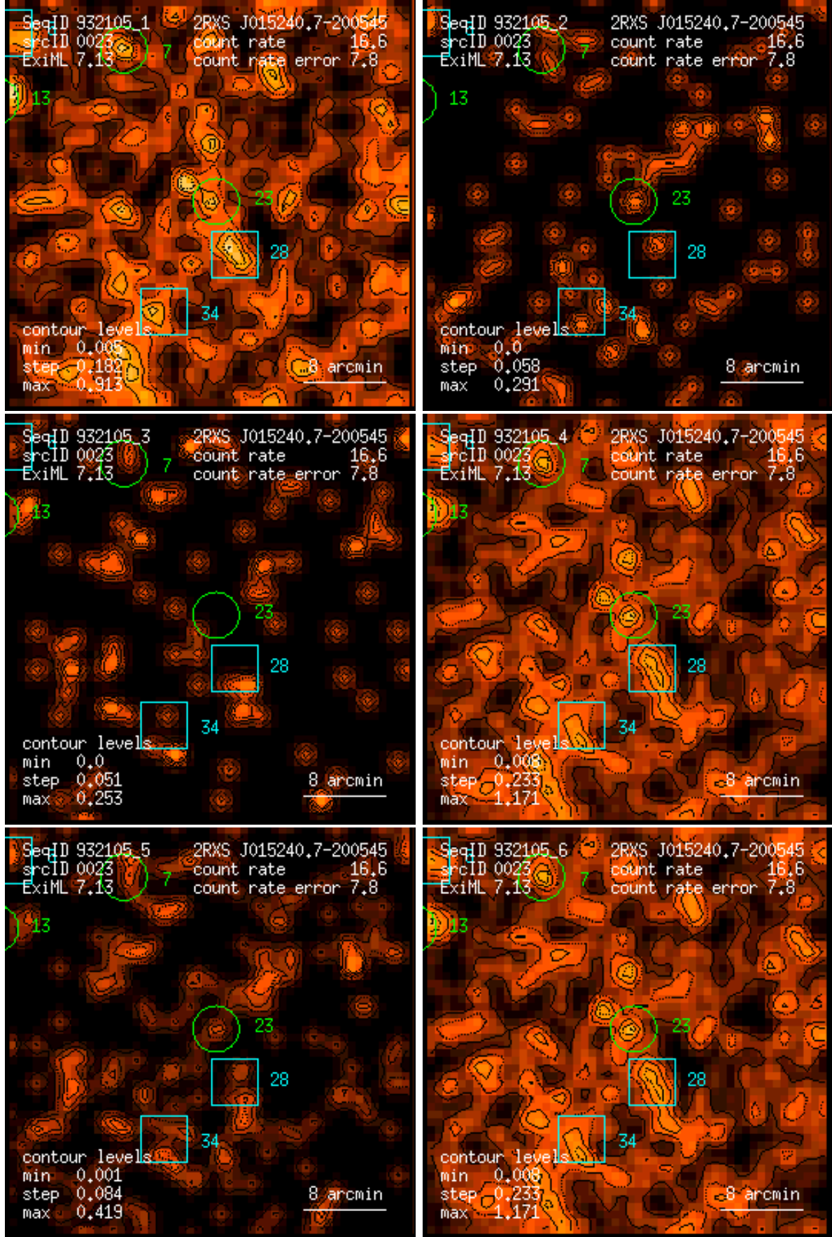
Figure 23: RASS 932105: detection 0023: band rate images, Gaussian filter: (1) PSPC channels 11 – 41, (2) 52 – 90, (3) 91 – 201, (4) 11 – 235, (5) 52 – 201, (6) 11 – 201. Broad band rates in counts/ks. Band rate contour levels in counts/ks/arcmin 2 .
