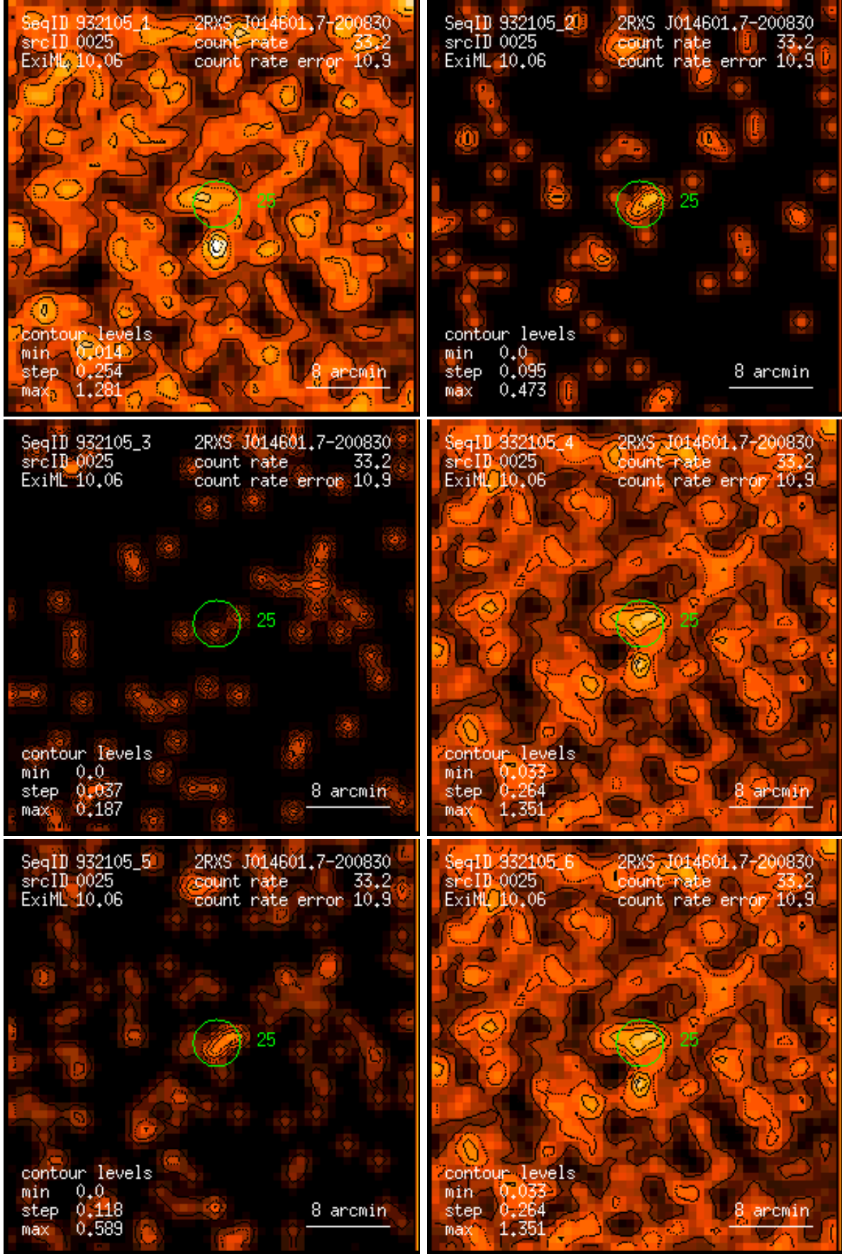
Figure 25: RASS 932105: detection 0025: band rate images, Gaussian filter: (1) PSPC channels 11 – 41, (2) 52 – 90, (3) 91 – 201, (4) 11 – 235, (5) 52 – 201, (6) 11 – 201. Broad band rates in counts/ks. Band rate contour levels in counts/ks/arcmin 2 .
