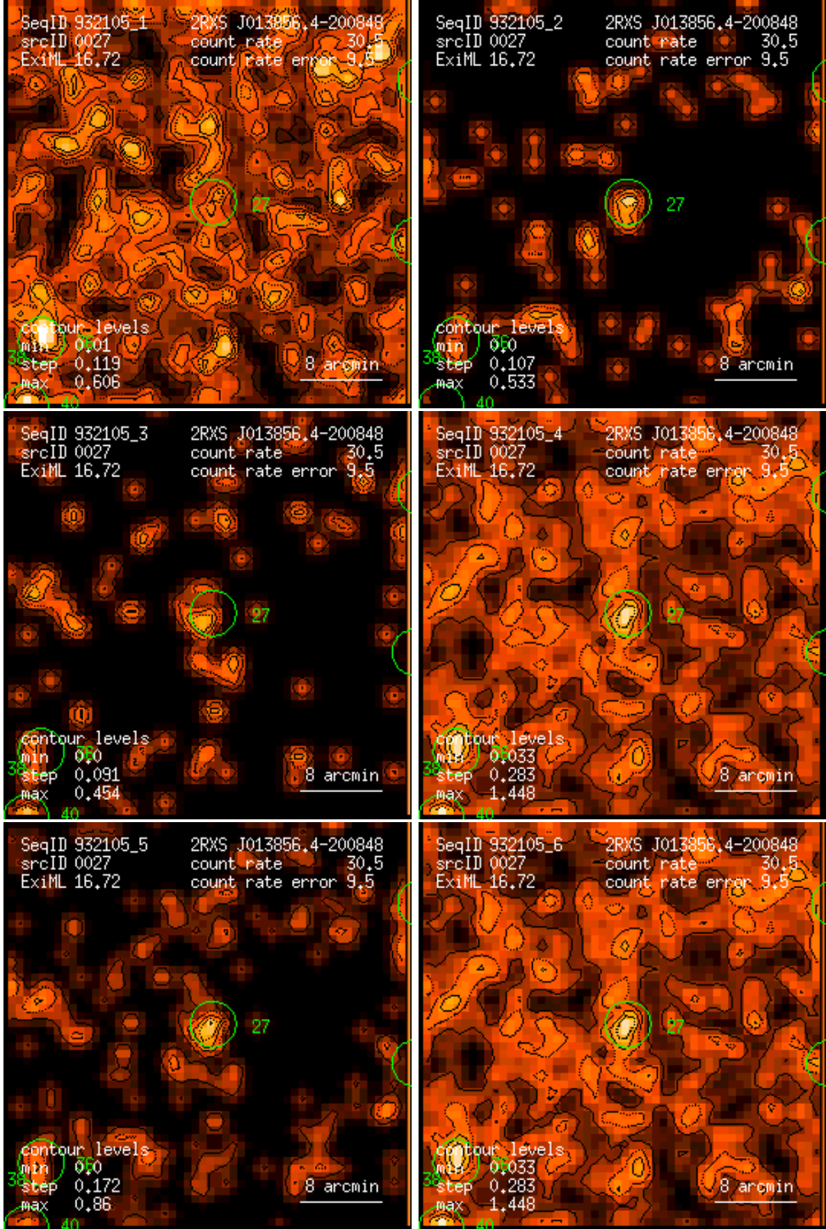
Figure 27: RASS 932105: detection 0027: band rate images, Gaussian filter: (1) PSPC channels 11 – 41, (2) 52 – 90, (3) 91 – 201, (4) 11 – 235, (5) 52 – 201, (6) 11 – 201. Broad band rates in counts/ks. Band rate contour levels in counts/ks/arcmin 2 .
