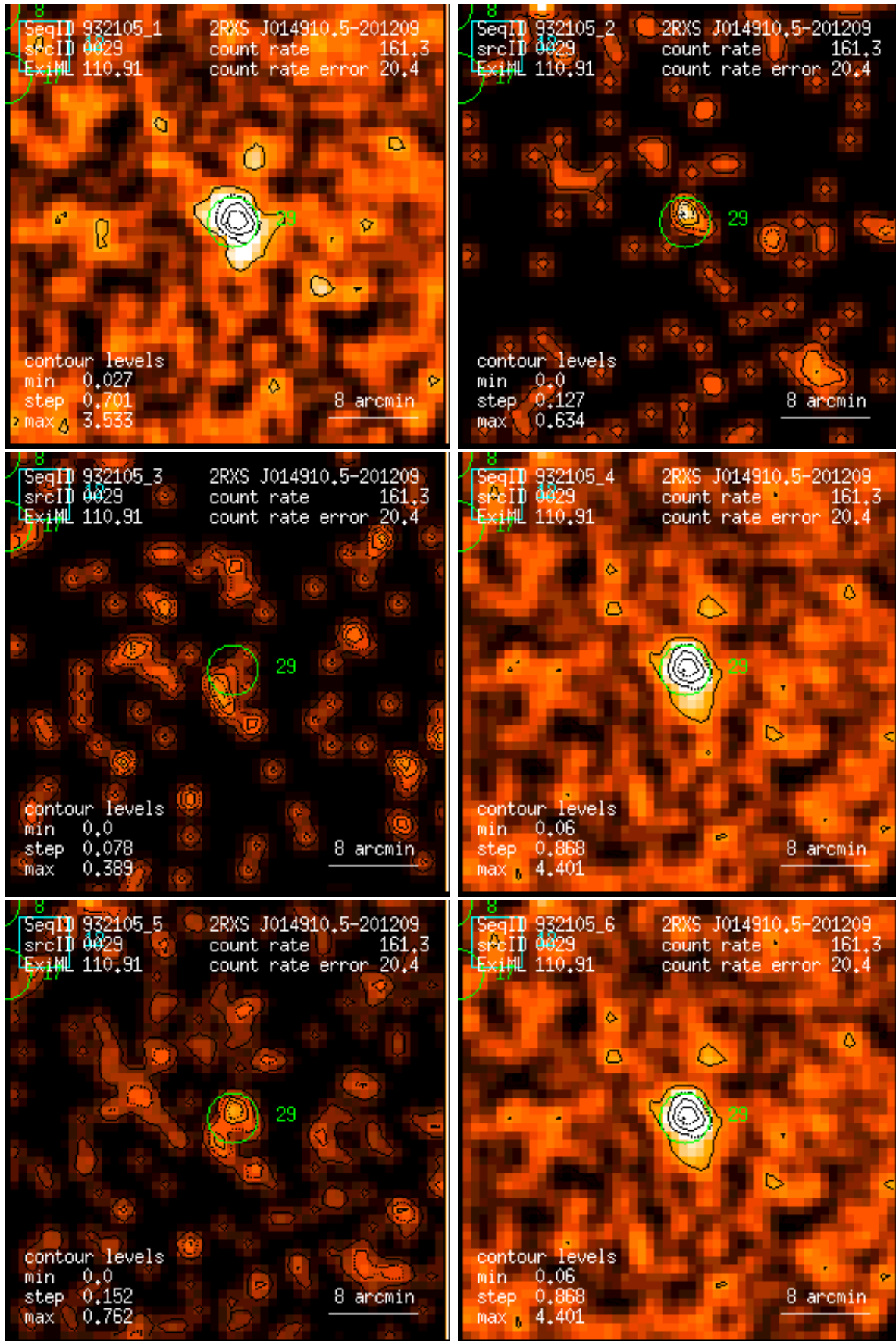
Figure 29: RASS 932105: detection 0029: band rate images, Gaussian filter: (1) PSPC channels 11 – 41, (2) 52 – 90, (3) 91 – 201, (4) 11 – 235, (5) 52 – 201, (6) 11 – 201. Broad band rates in counts/ks. Band rate contour levels in counts/ks/arcmin 2 .
