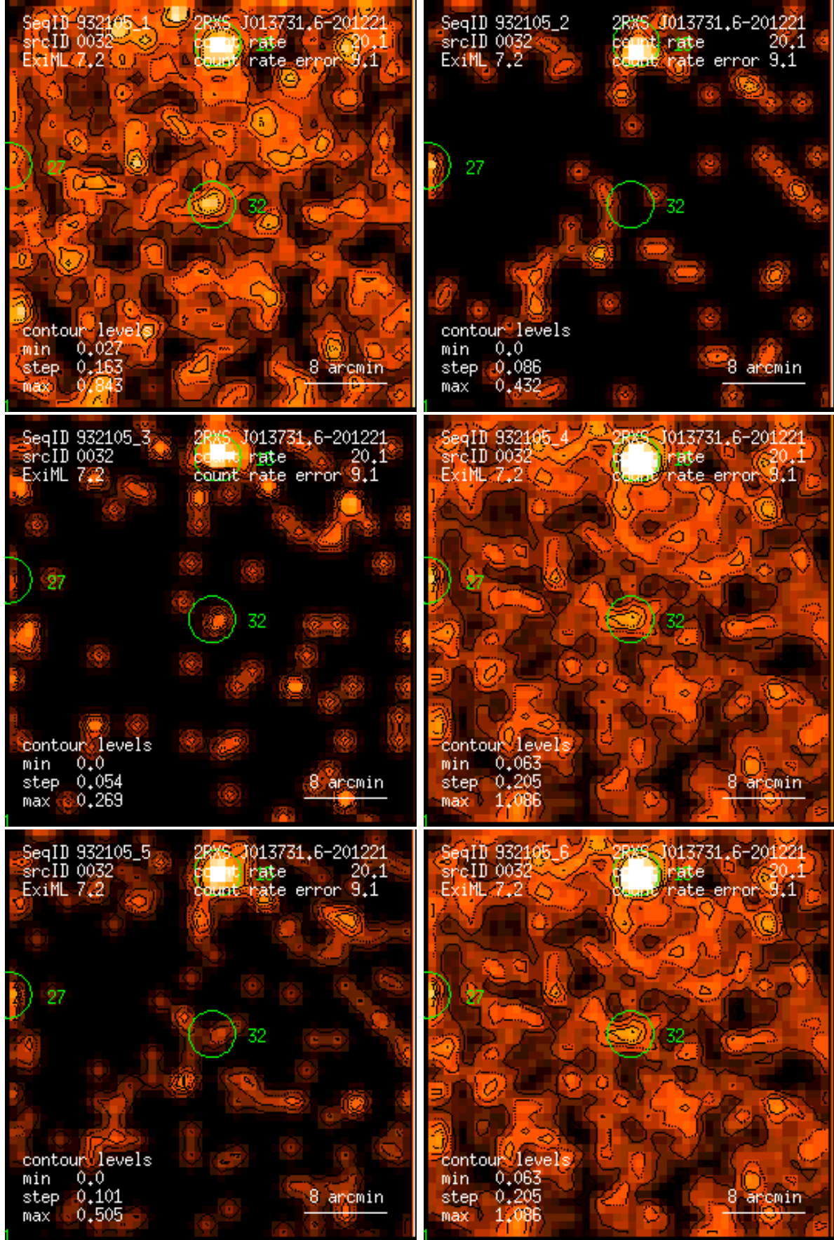
Figure 32: RASS 932105: detection 0032: band rate images, Gaussian filter: (1) PSPC channels 11 – 41, (2) 52 – 90, (3) 91 – 201, (4) 11 – 235, (5) 52 – 201, (6) 11 – 201. Broad band rates in counts/ks. Band rate contour levels in counts/ks/arcmin 2 .
