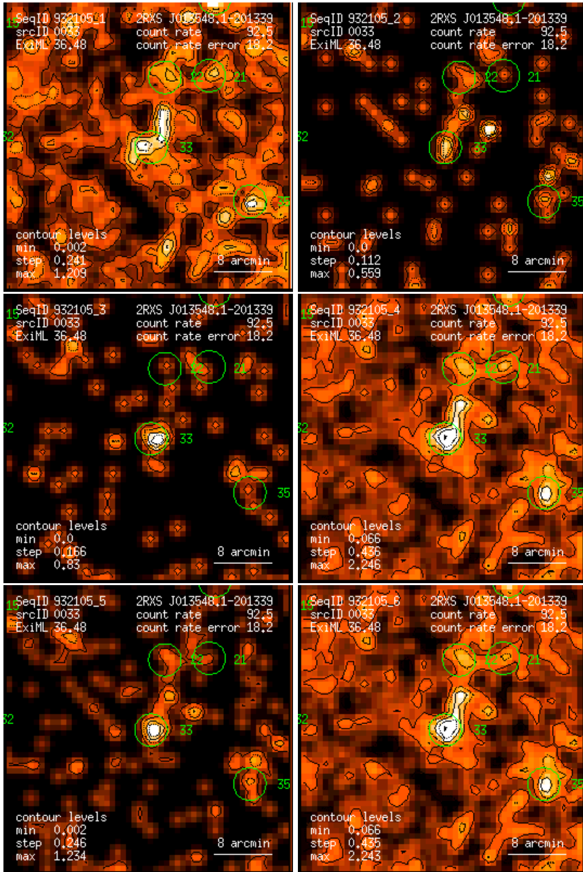
Figure 33: RASS 932105: detection 0033: band rate images, Gaussian filter: (1) PSPC channels 11 – 41, (2) 52 – 90, (3) 91 – 201, (4) 11 – 235, (5) 52 – 201, (6) 11 – 201. Broad band rates in counts/ks. Band rate contour levels in counts/ks/arcmin 2 .
