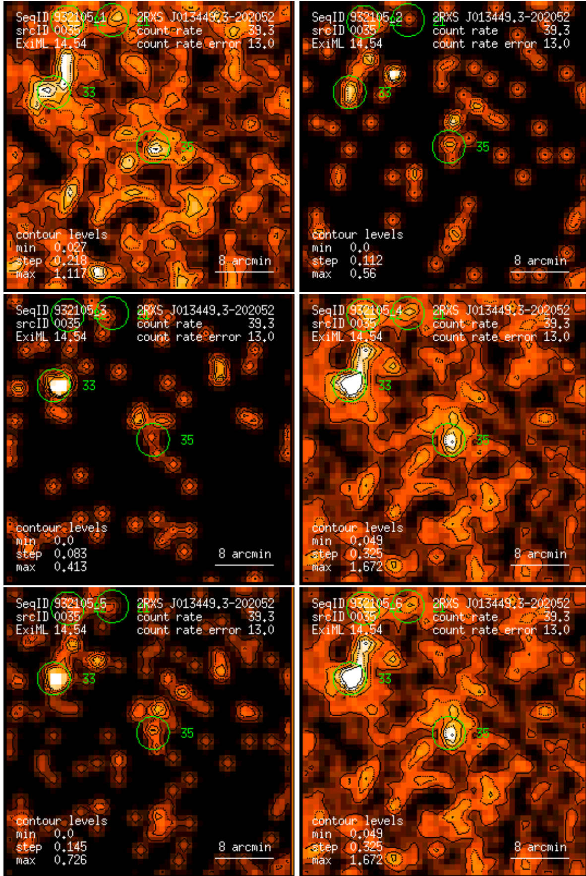
Figure 35: RASS 932105: detection 0035: band rate images, Gaussian filter: (1) PSPC channels 11 – 41, (2) 52 – 90, (3) 91 – 201, (4) 11 – 235, (5) 52 – 201, (6) 11 – 201. Broad band rates in counts/ks. Band rate contour levels in counts/ks/arcmin 2 .
