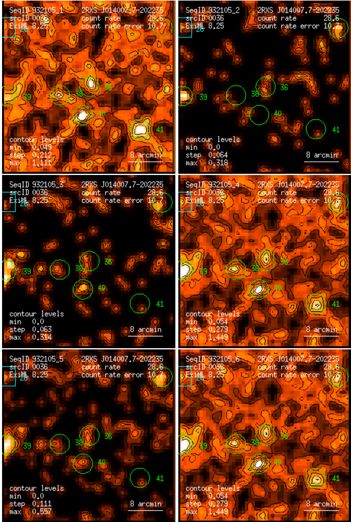
Figure 36: RASS 932105: detection 0036: band rate images, Gaussian filter: (1) PSPC channels 11 – 41, (2) 52 – 90, (3) 91 – 201, (4) 11 – 235, (5) 52 – 201, (6) 11 – 201. Broad band rates in counts/ks. Band rate contour levels in counts/ks/arcmin 2 .
