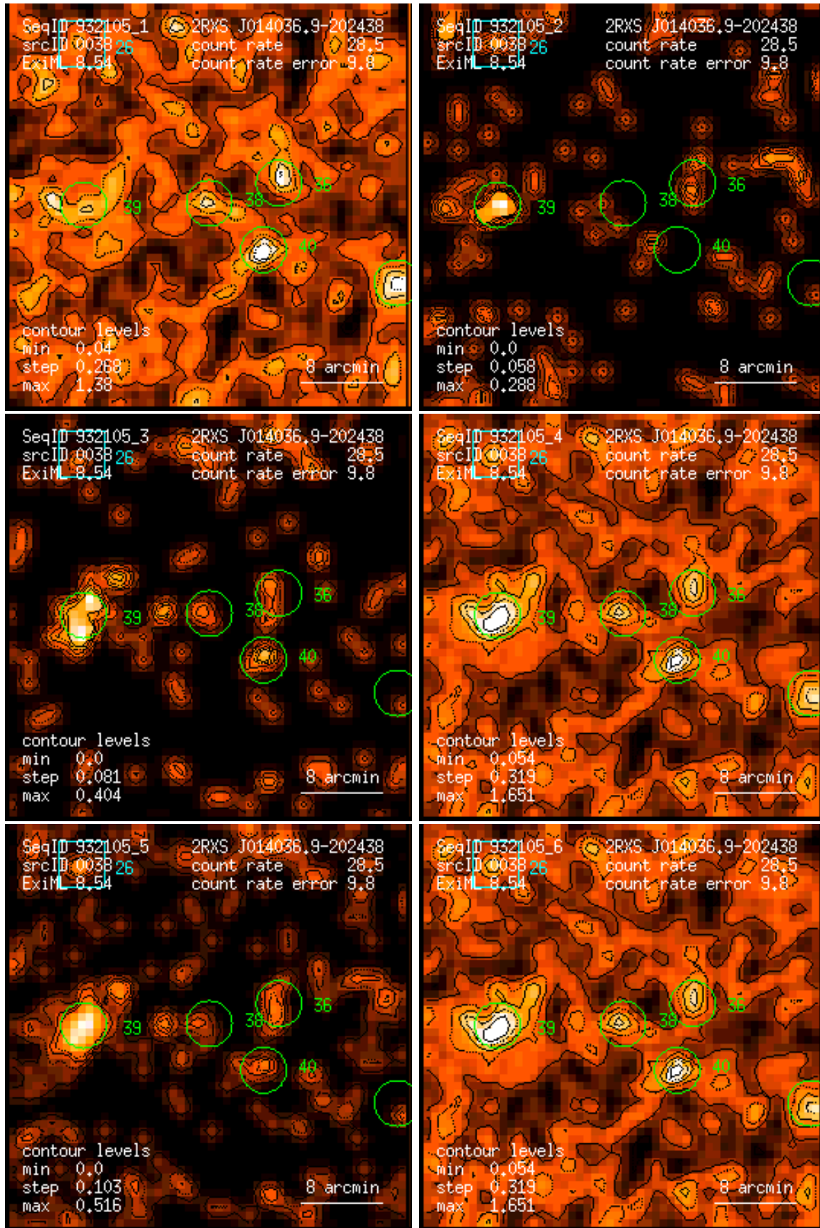
Figure 38: RASS 932105: detection 0038: band rate images, Gaussian filter: (1) PSPC channels 11 – 41, (2) 52 – 90, (3) 91 – 201, (4) 11 – 235, (5) 52 – 201, (6) 11 – 201. Broad band rates in counts/ks. Band rate contour levels in counts/ks/arcmin 2 .
