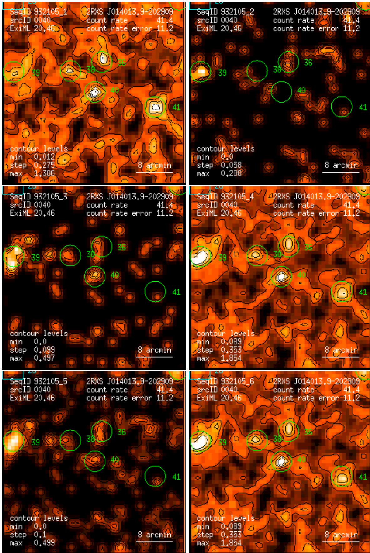
Figure 40: RASS 932105: detection 0040: band rate images, Gaussian filter: (1) PSPC channels 11 – 41, (2) 52 – 90, (3) 91 – 201, (4) 11 – 235, (5) 52 – 201, (6) 11 – 201. Broad band rates in counts/ks. Band rate contour levels in counts/ks/arcmin 2 .
