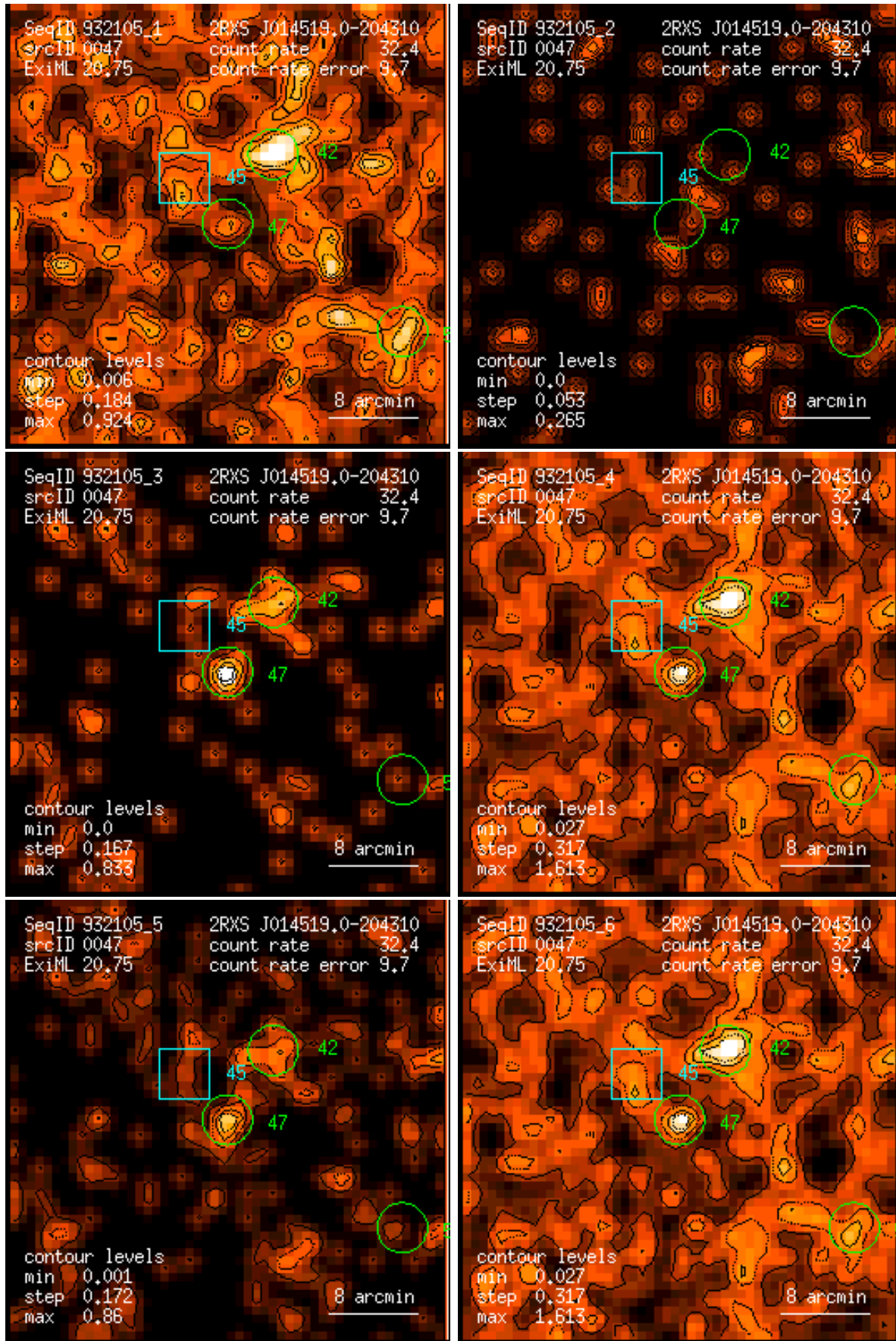
Figure 47: RASS 932105: detection 0047: band rate images, Gaussian filter: (1) PSPC channels 11 – 41, (2) 52 – 90, (3) 91 – 201, (4) 11 – 235, (5) 52 – 201, (6) 11 – 201. Broad band rates in counts/ks. Band rate contour levels in counts/ks/arcmin 2 .
