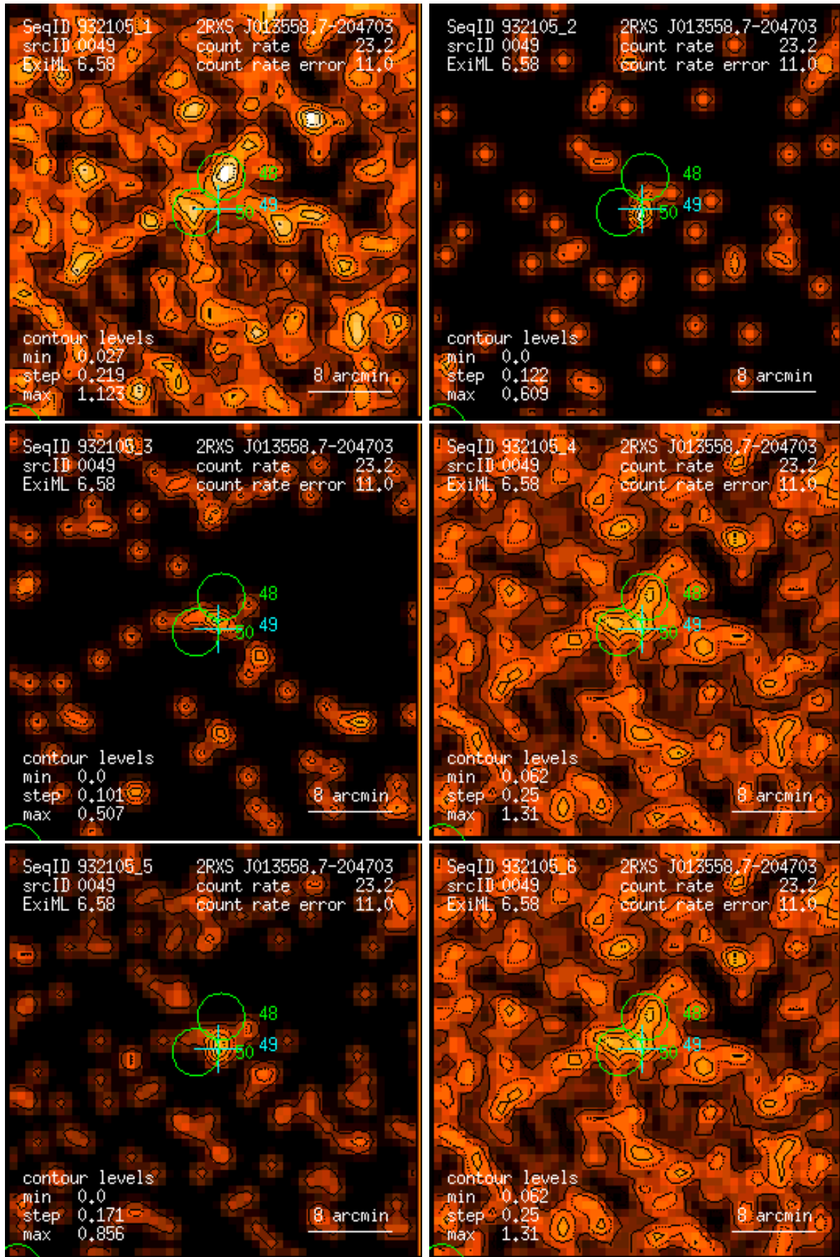
Figure 49: RASS 932105: detection 0049: band rate images, Gaussian filter: (1) PSPC channels 11 – 41, (2) 52 – 90, (3) 91 – 201, (4) 11 – 235, (5) 52 – 201, (6) 11 – 201. Broad band rates in counts/ks. Band rate contour levels in counts/ks/arcmin 2 .
