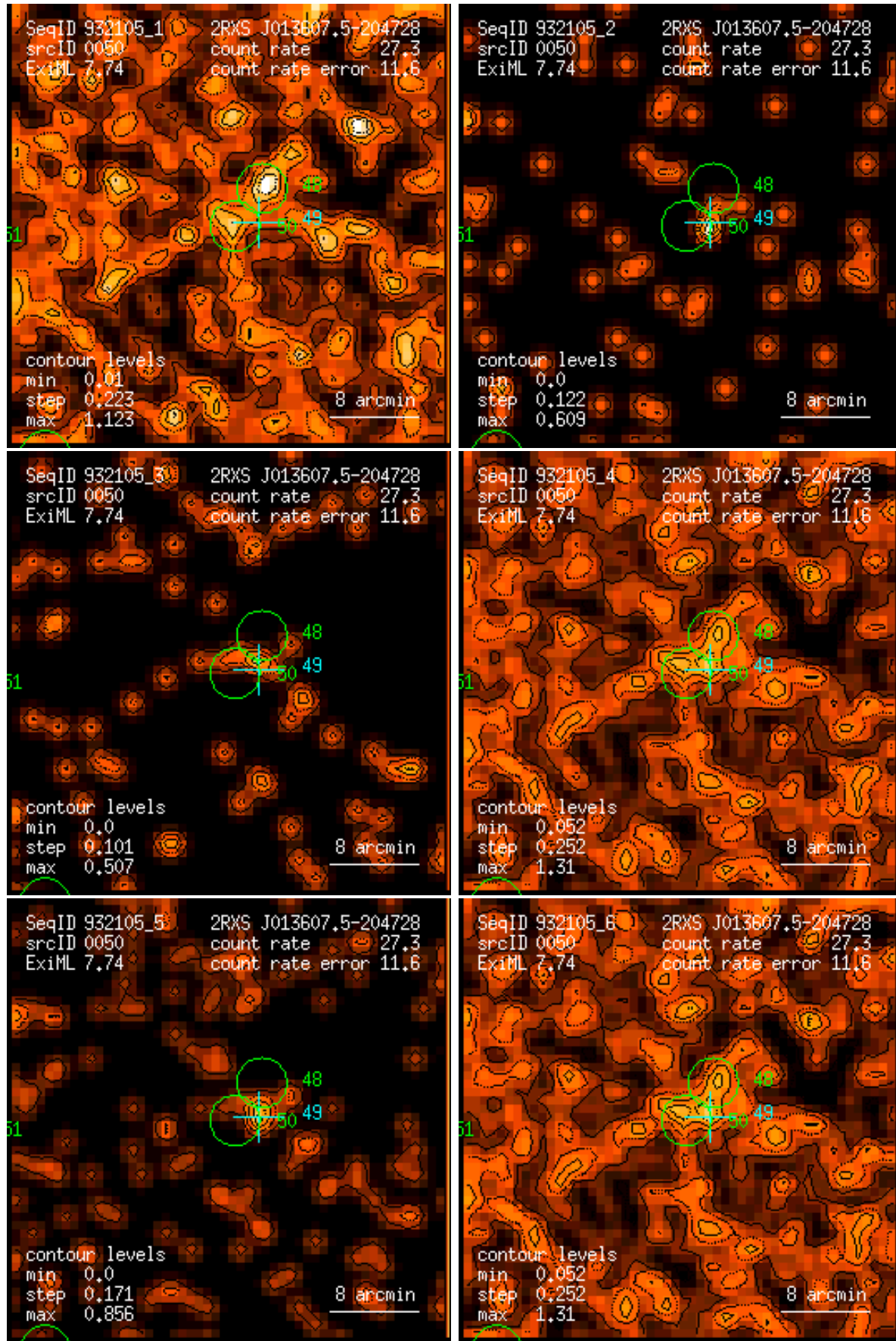
Figure 50: RASS 932105: detection 0050: band rate images, Gaussian filter: (1) PSPC channels 11 – 41, (2) 52 – 90, (3) 91 – 201, (4) 11 – 235, (5) 52 – 201, (6) 11 – 201. Broad band rates in counts/ks. Band rate contour levels in counts/ks/arcmin 2 .
