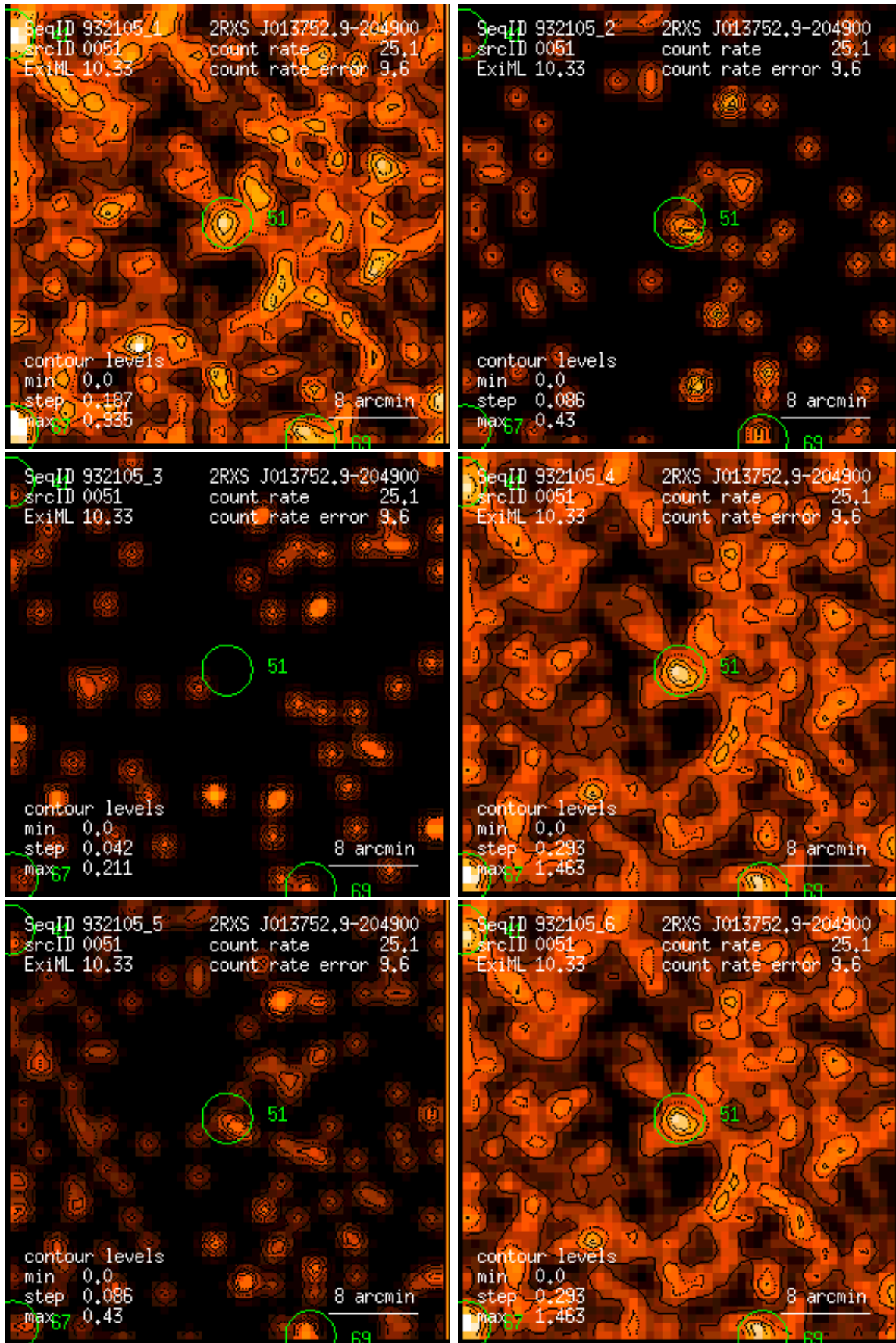
Figure 51: RASS 932105: detection 0051: band rate images, Gaussian filter: (1) PSPC channels 11 – 41, (2) 52 – 90, (3) 91 – 201, (4) 11 – 235, (5) 52 – 201, (6) 11 – 201. Broad band rates in counts/ks. Band rate contour levels in counts/ks/arcmin 2 .
