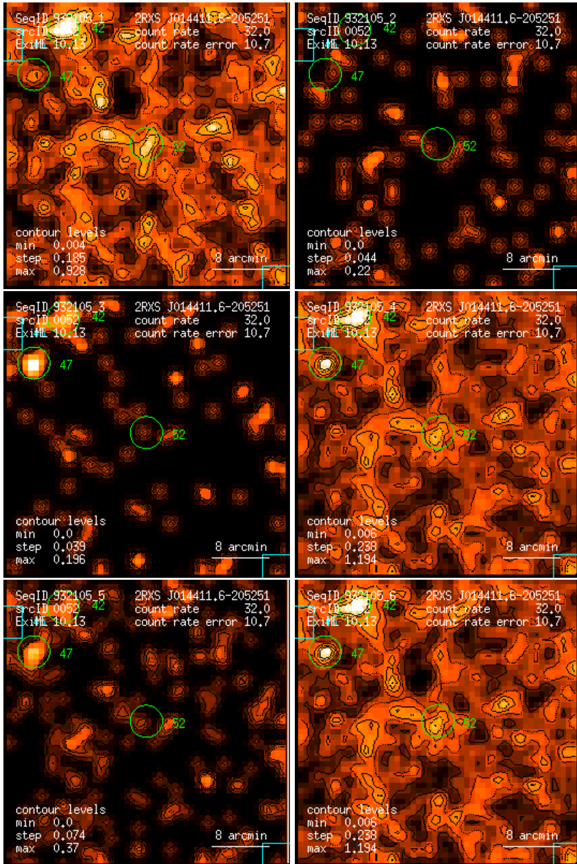
Figure 52: RASS 932105: detection 0052: band rate images, Gaussian filter: (1) PSPC channels 11 – 41, (2) 52 – 90, (3) 91 – 201, (4) 11 – 235, (5) 52 – 201, (6) 11 – 201. Broad band rates in counts/ks. Band rate contour levels in counts/ks/arcmin 2 .
