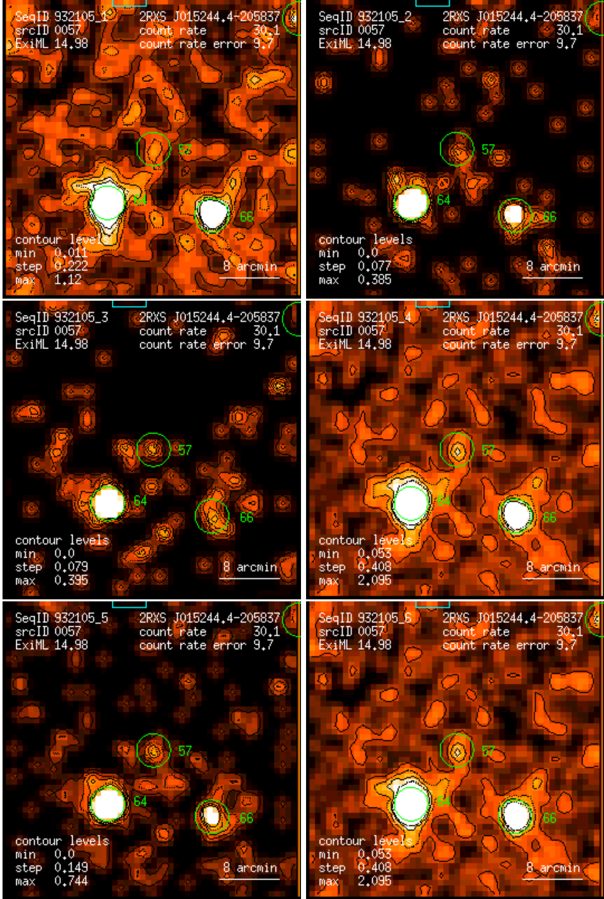
Figure 57: RASS 932105: detection 0057: band rate images, Gaussian filter: (1) PSPC channels 11 – 41, (2) 52 – 90, (3) 91 – 201, (4) 11 – 235, (5) 52 – 201, (6) 11 – 201. Broad band rates in counts/ks. Band rate contour levels in counts/ks/arcmin 2 .
