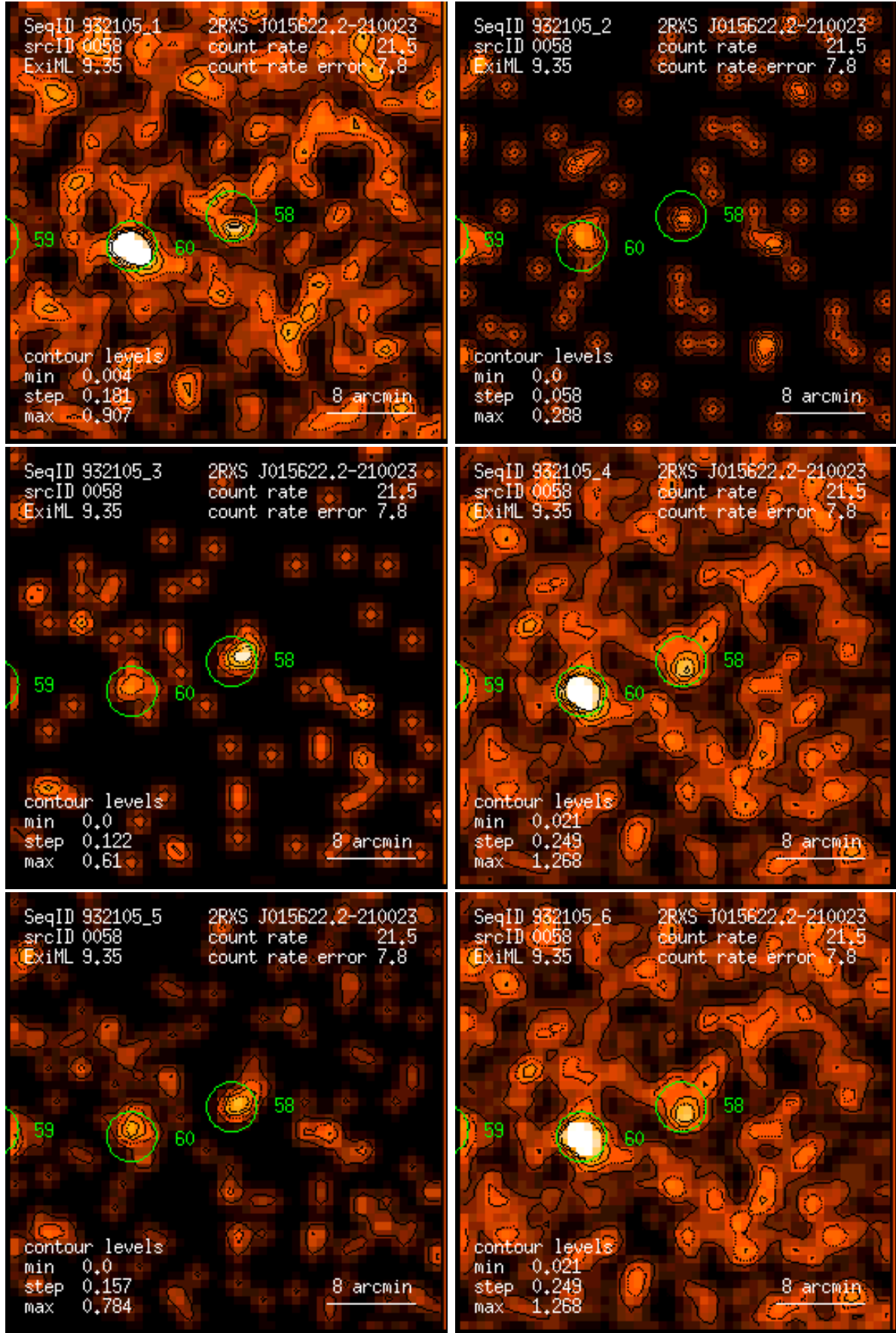
Figure 58: RASS 932105: detection 0058: band rate images, Gaussian filter: (1) PSPC channels 11 – 41, (2) 52 – 90, (3) 91 – 201, (4) 11 – 235, (5) 52 – 201, (6) 11 – 201. Broad band rates in counts/ks. Band rate contour levels in counts/ks/arcmin 2 .
