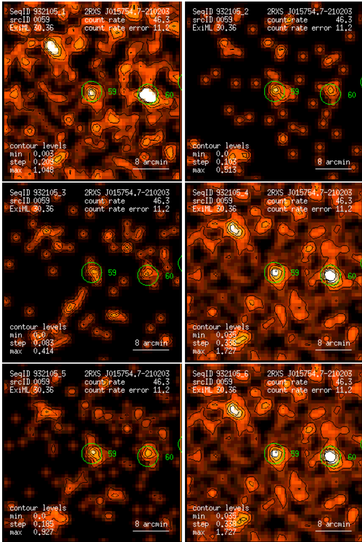
Figure 59: RASS 932105: detection 0059: band rate images, Gaussian filter: (1) PSPC channels 11 – 41, (2) 52 – 90, (3) 91 – 201, (4) 11 – 235, (5) 52 – 201, (6) 11 – 201. Broad band rates in counts/ks. Band rate contour levels in counts/ks/arcmin 2 .
