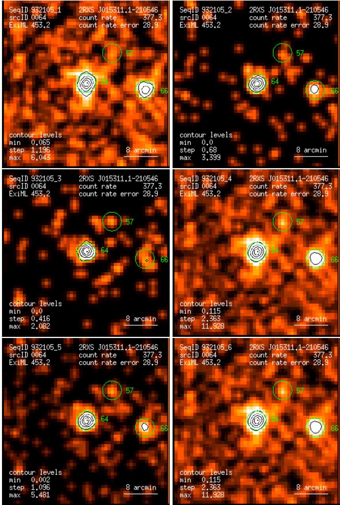
Figure 64: RASS 932105: detection 0064: band rate images, Gaussian filter: (1) PSPC channels 11 – 41, (2) 52 – 90, (3) 91 – 201, (4) 11 – 235, (5) 52 – 201, (6) 11 – 201. Broad band rates in counts/ks. Band rate contour levels in counts/ks/arcmin 2 .
