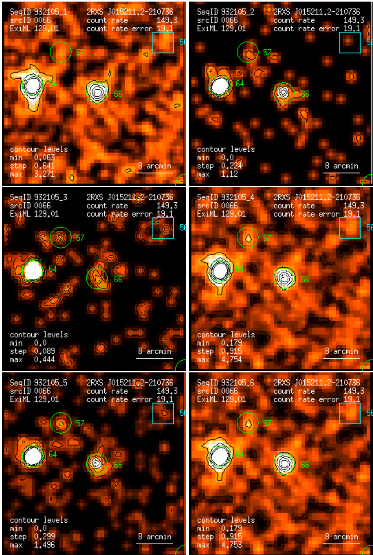
Figure 66: RASS 932105: detection 0066: band rate images, Gaussian filter: (1) PSPC channels 11 – 41, (2) 52 – 90, (3) 91 – 201, (4) 11 – 235, (5) 52 – 201, (6) 11 – 201. Broad band rates in counts/ks. Band rate contour levels in counts/ks/arcmin 2 .
