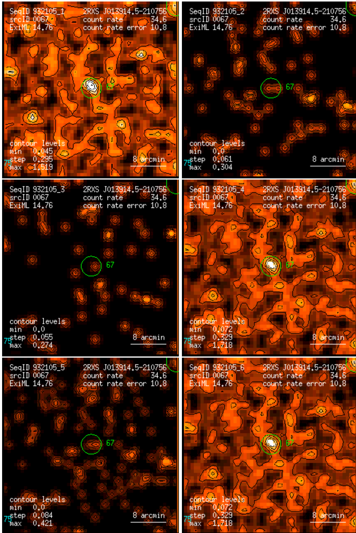
Figure 67: RASS 932105: detection 0067: band rate images, Gaussian filter: (1) PSPC channels 11 – 41, (2) 52 – 90, (3) 91 – 201, (4) 11 – 235, (5) 52 – 201, (6) 11 – 201. Broad band rates in counts/ks. Band rate contour levels in counts/ks/arcmin 2 .
