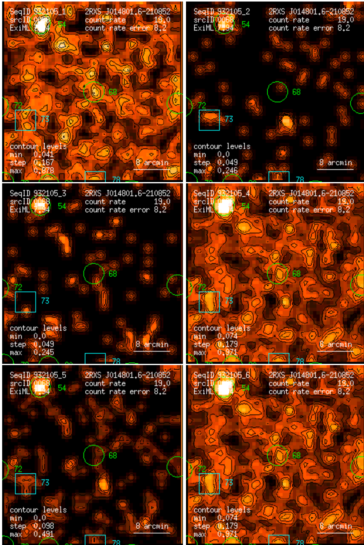
Figure 68: RASS 932105: detection 0068: band rate images, Gaussian filter: (1) PSPC channels 11 – 41, (2) 52 – 90, (3) 91 – 201, (4) 11 – 235, (5) 52 – 201, (6) 11 – 201. Broad band rates in counts/ks. Band rate contour levels in counts/ks/arcmin 2 .
