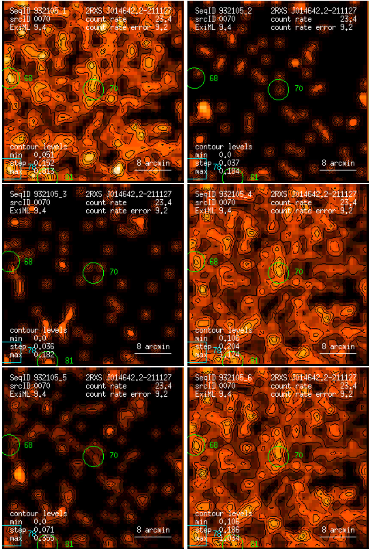
Figure 70: RASS 932105: detection 0070: band rate images, Gaussian filter: (1) PSPC channels 11 – 41, (2) 52 – 90, (3) 91 – 201, (4) 11 – 235, (5) 52 – 201, (6) 11 – 201. Broad band rates in counts/ks. Band rate contour levels in counts/ks/arcmin 2 .
