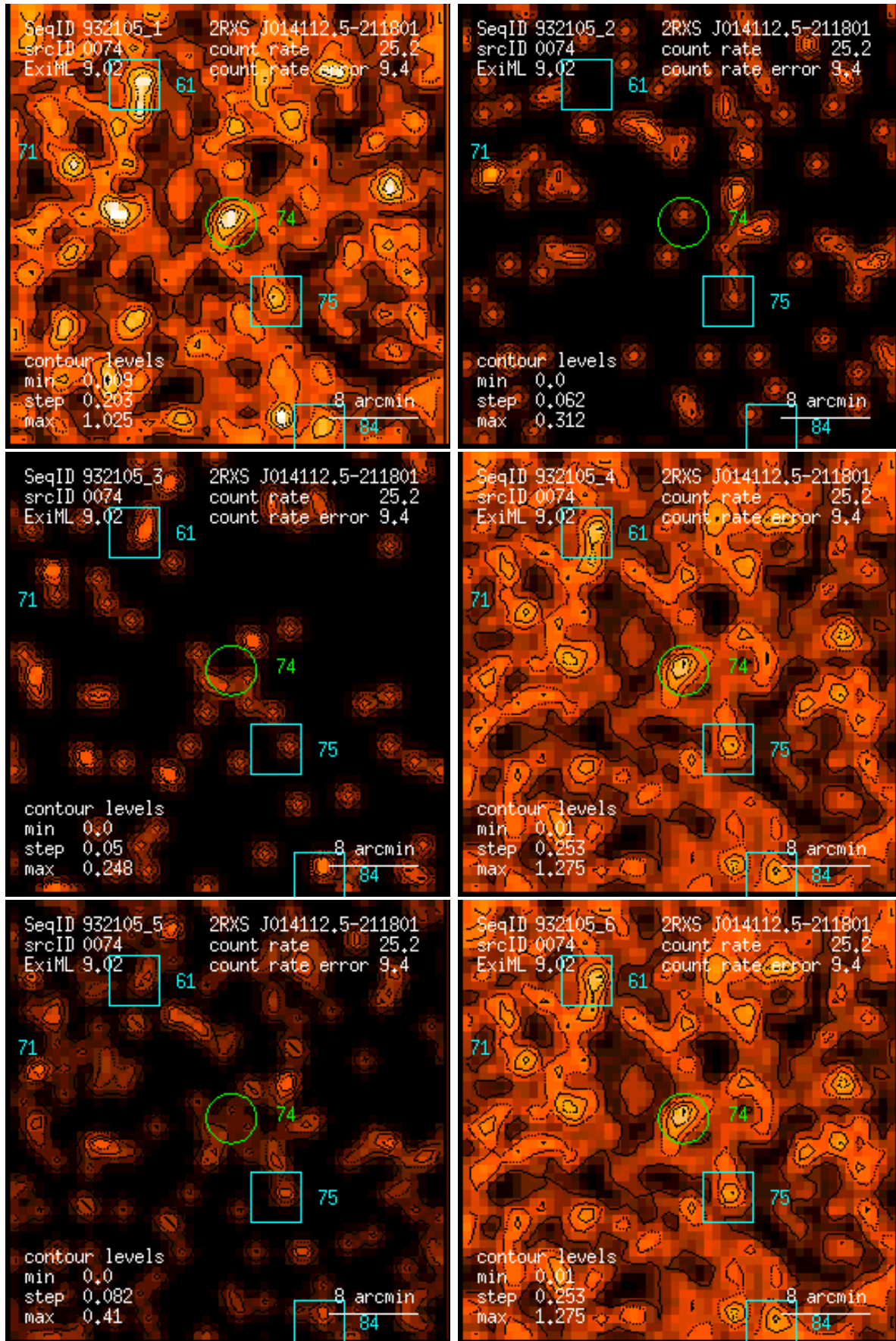
Figure 74: RASS 932105: detection 0074: band rate images, Gaussian filter: (1) PSPC channels 11 – 41, (2) 52 – 90, (3) 91 – 201, (4) 11 – 235, (5) 52 – 201, (6) 11 – 201. Broad band rates in counts/ks. Band rate contour levels in counts/ks/arcmin 2 .
