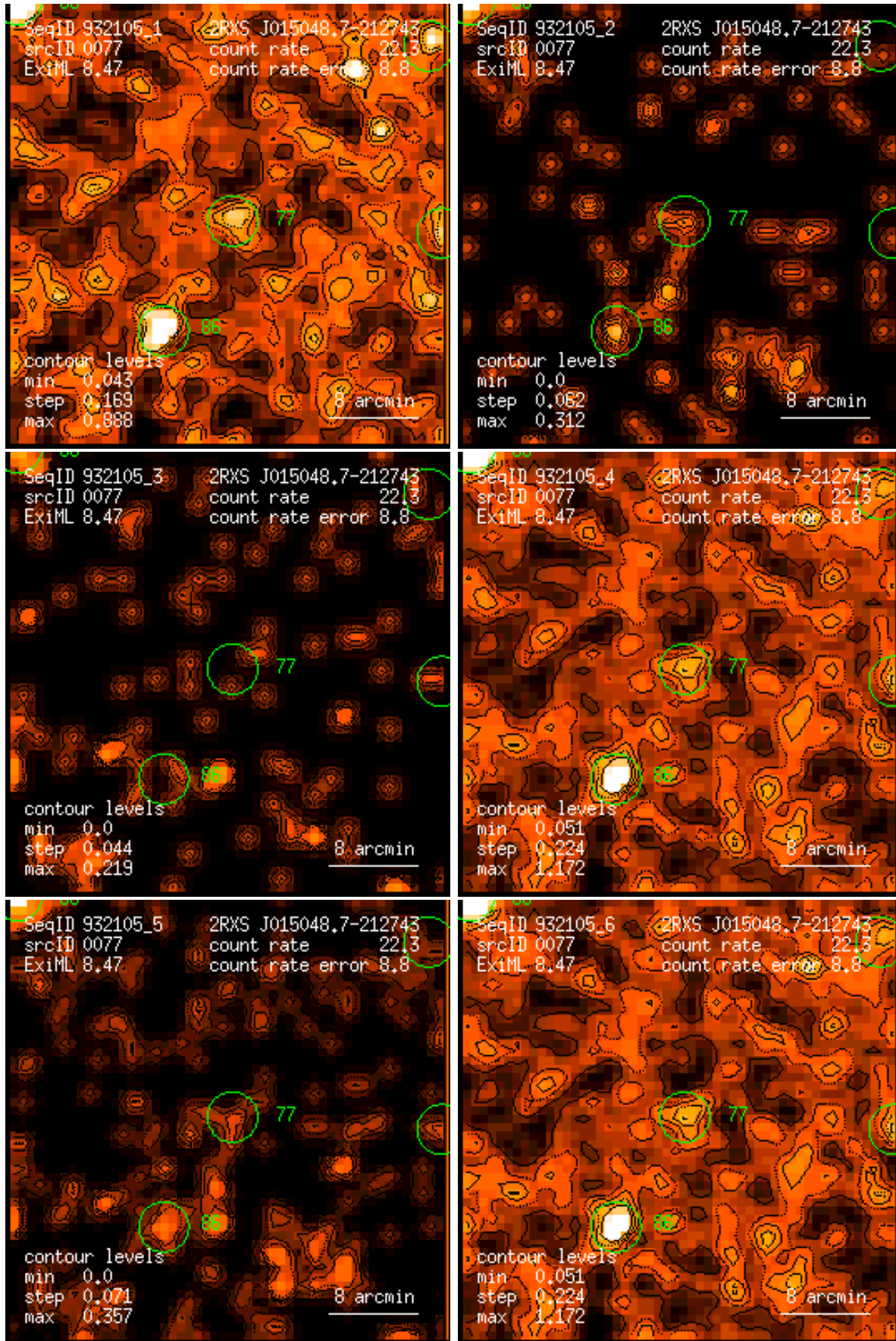
Figure 77: RASS 932105: detection 0077: band rate images, Gaussian filter: (1) PSPC channels 11 – 41, (2) 52 – 90, (3) 91 – 201, (4) 11 – 235, (5) 52 – 201, (6) 11 – 201. Broad band rates in counts/ks. Band rate contour levels in counts/ks/arcmin 2 .
