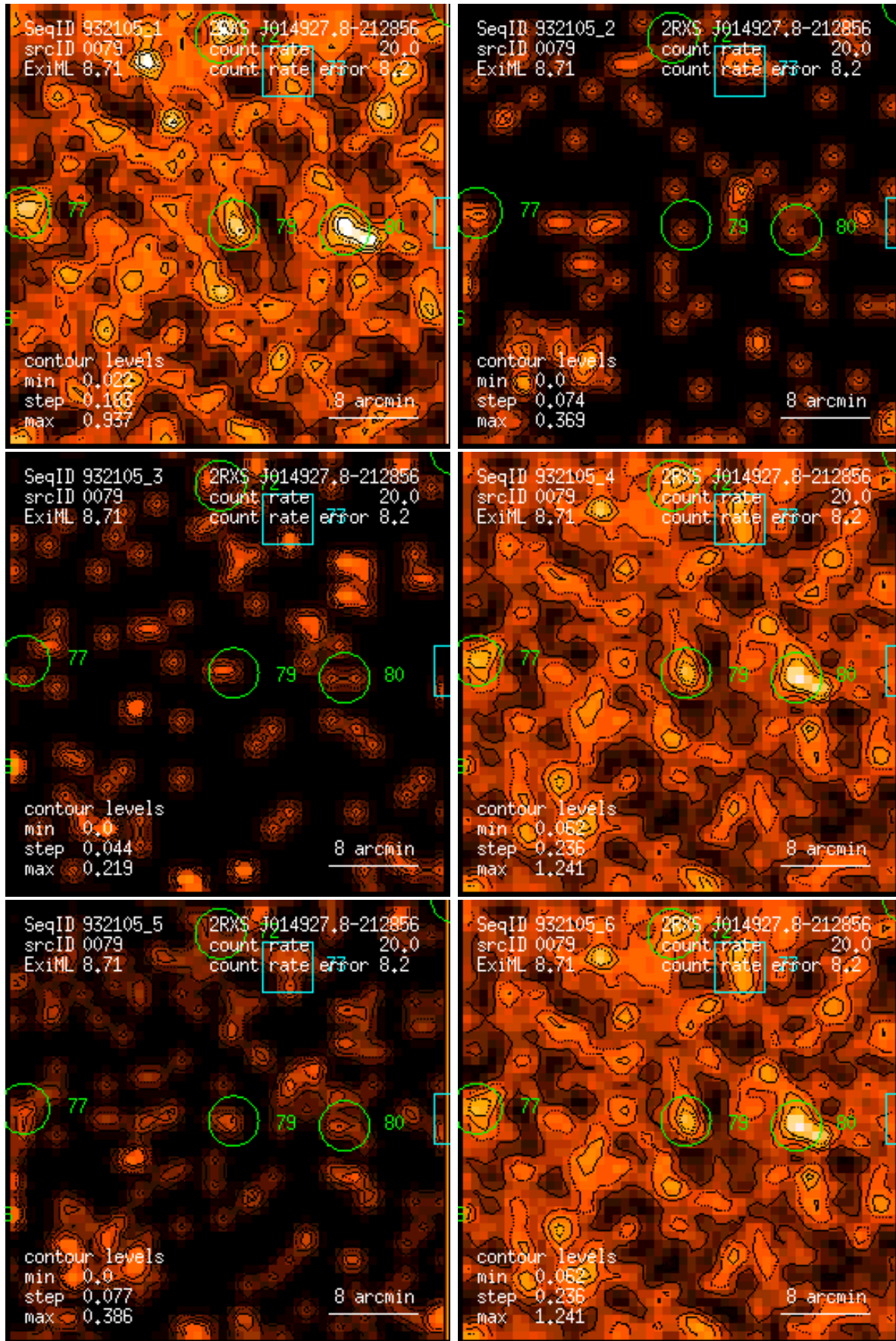
Figure 79: RASS 932105: detection 0079: band rate images, Gaussian filter: (1) PSPC channels 11 – 41, (2) 52 – 90, (3) 91 – 201, (4) 11 – 235, (5) 52 – 201, (6) 11 – 201. Broad band rates in counts/ks. Band rate contour levels in counts/ks/arcmin 2 .
