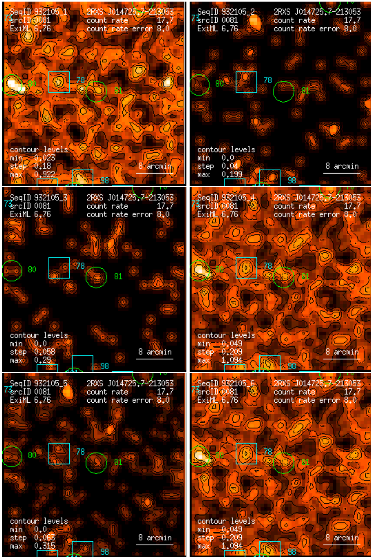
Figure 81: RASS 932105: detection 0081: band rate images, Gaussian filter: (1) PSPC channels 11 – 41, (2) 52 – 90, (3) 91 – 201, (4) 11 – 235, (5) 52 – 201, (6) 11 – 201. Broad band rates in counts/ks. Band rate contour levels in counts/ks/arcmin 2 .
