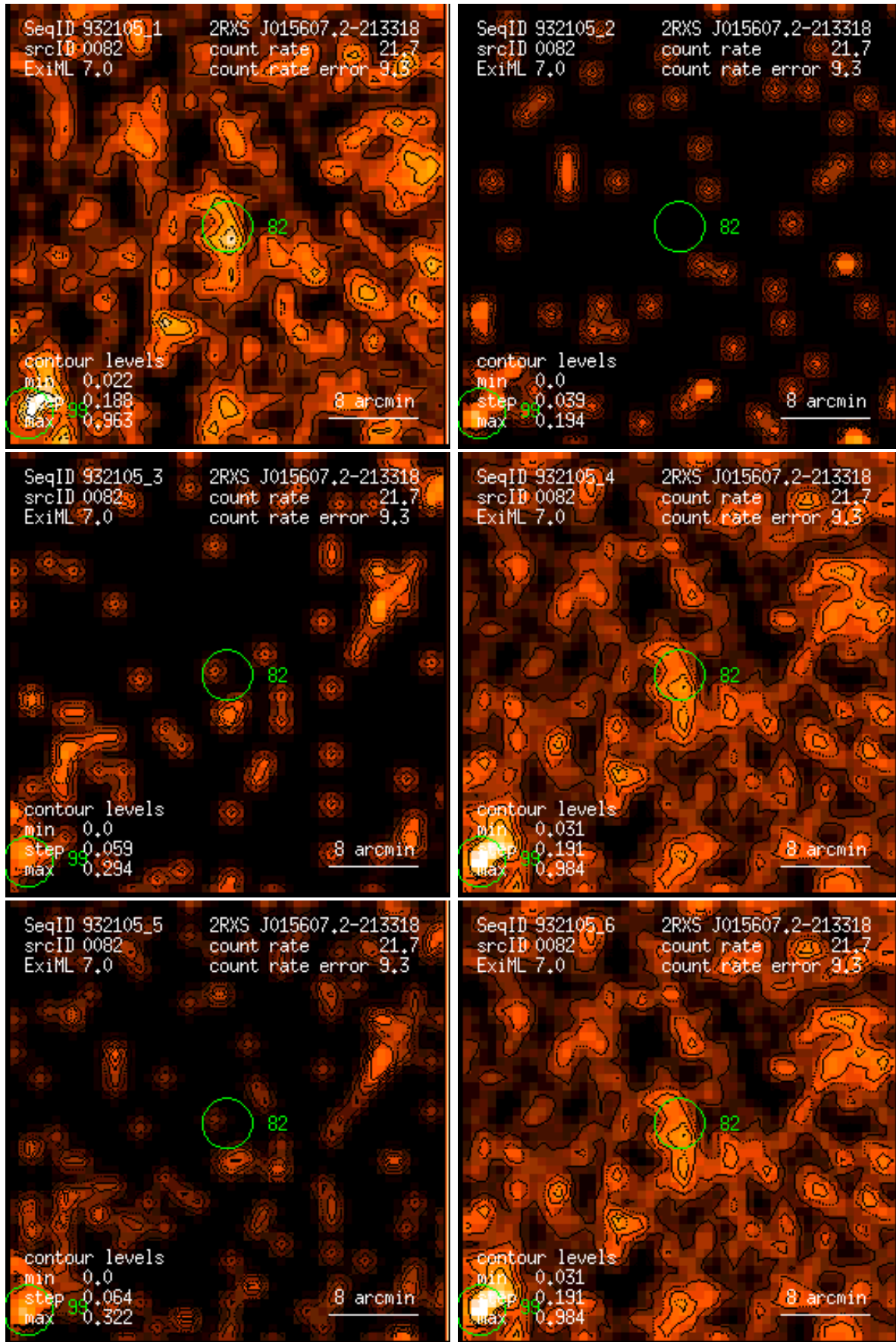
Figure 82: RASS 932105: detection 0082: band rate images, Gaussian filter: (1) PSPC channels 11 – 41, (2) 52 – 90, (3) 91 – 201, (4) 11 – 235, (5) 52 – 201, (6) 11 – 201. Broad band rates in counts/ks. Band rate contour levels in counts/ks/arcmin 2 .
