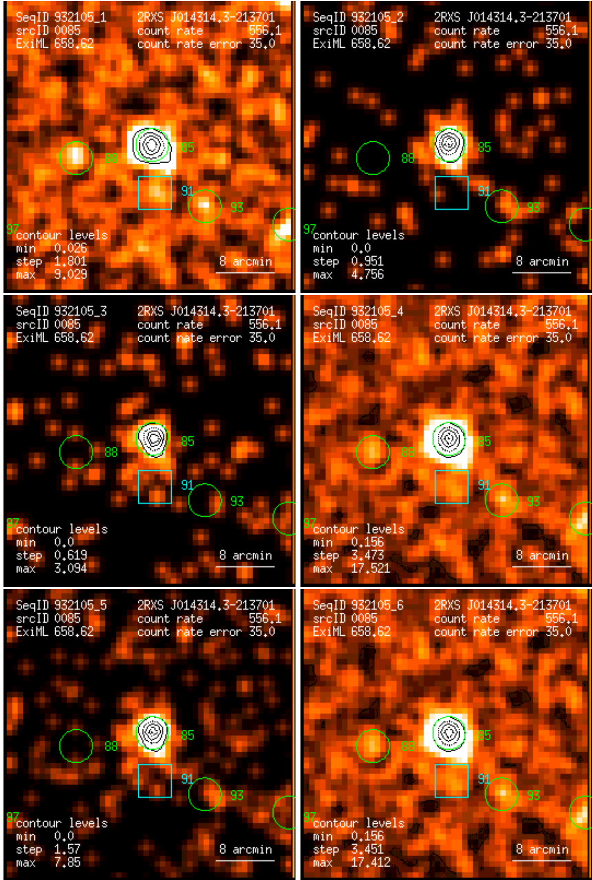
Figure 85: RASS 932105: detection 0085: band rate images, Gaussian filter: (1) PSPC channels 11 – 41, (2) 52 – 90, (3) 91 – 201, (4) 11 – 235, (5) 52 – 201, (6) 11 – 201. Broad band rates in counts/ks. Band rate contour levels in counts/ks/arcmin 2 .
