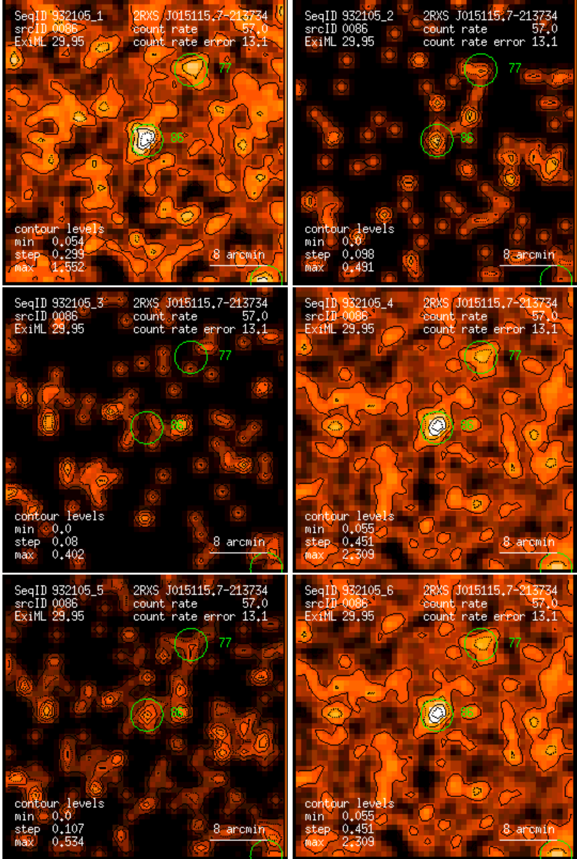
Figure 86: RASS 932105: detection 0086: band rate images, Gaussian filter: (1) PSPC channels 11 – 41, (2) 52 – 90, (3) 91 – 201, (4) 11 – 235, (5) 52 – 201, (6) 11 – 201. Broad band rates in counts/ks. Band rate contour levels in counts/ks/arcmin 2 .
