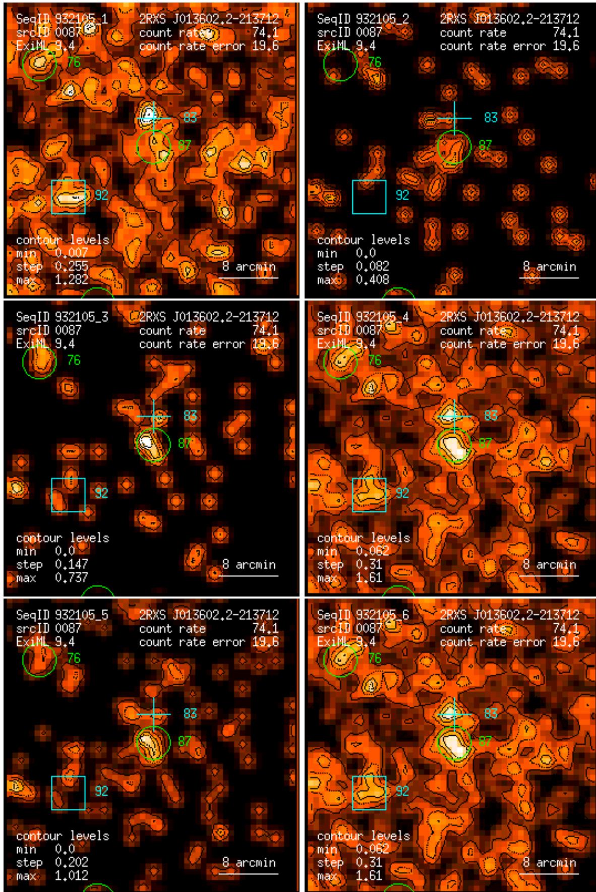
Figure 87: RASS 932105: detection 0087: band rate images, Gaussian filter: (1) PSPC channels 11 – 41, (2) 52 – 90, (3) 91 – 201, (4) 11 – 235, (5) 52 – 201, (6) 11 – 201. Broad band rates in counts/ks. Band rate contour levels in counts/ks/arcmin 2 .
