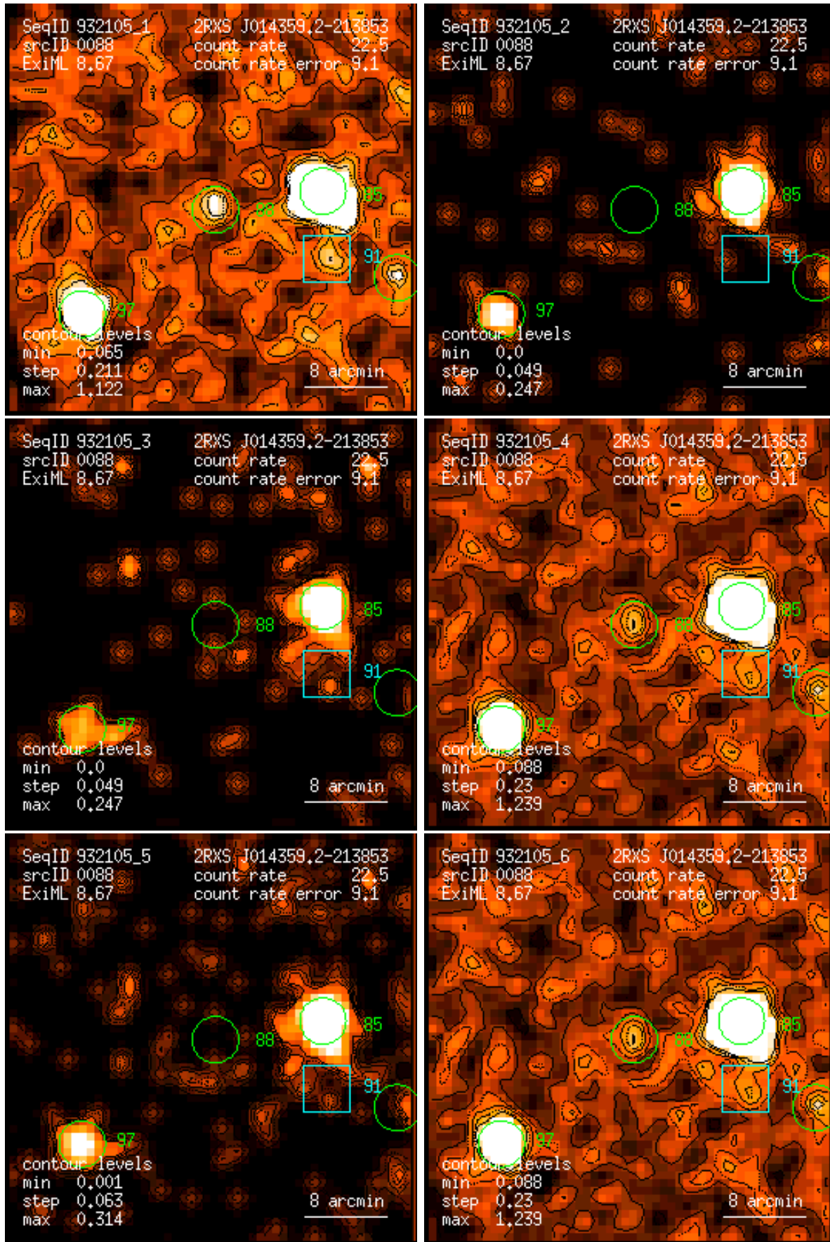
Figure 88: RASS 932105: detection 0088: band rate images, Gaussian filter: (1) PSPC channels 11 – 41, (2) 52 – 90, (3) 91 – 201, (4) 11 – 235, (5) 52 – 201, (6) 11 – 201. Broad band rates in counts/ks. Band rate contour levels in counts/ks/arcmin 2 .
