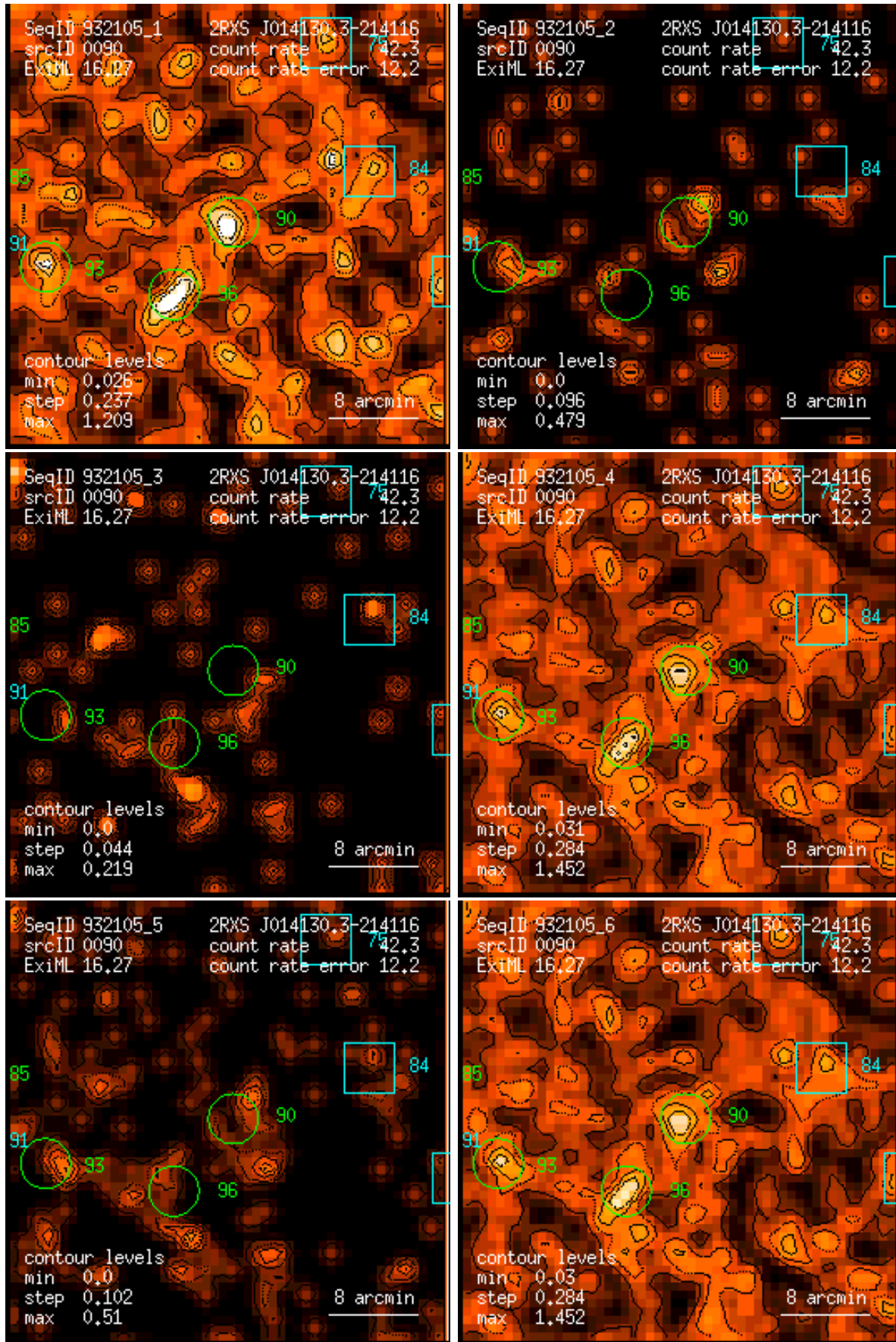
Figure 90: RASS 932105: detection 0090: band rate images, Gaussian filter: (1) PSPC channels 11 – 41, (2) 52 – 90, (3) 91 – 201, (4) 11 – 235, (5) 52 – 201, (6) 11 – 201. Broad band rates in counts/ks. Band rate contour levels in counts/ks/arcmin 2 .
