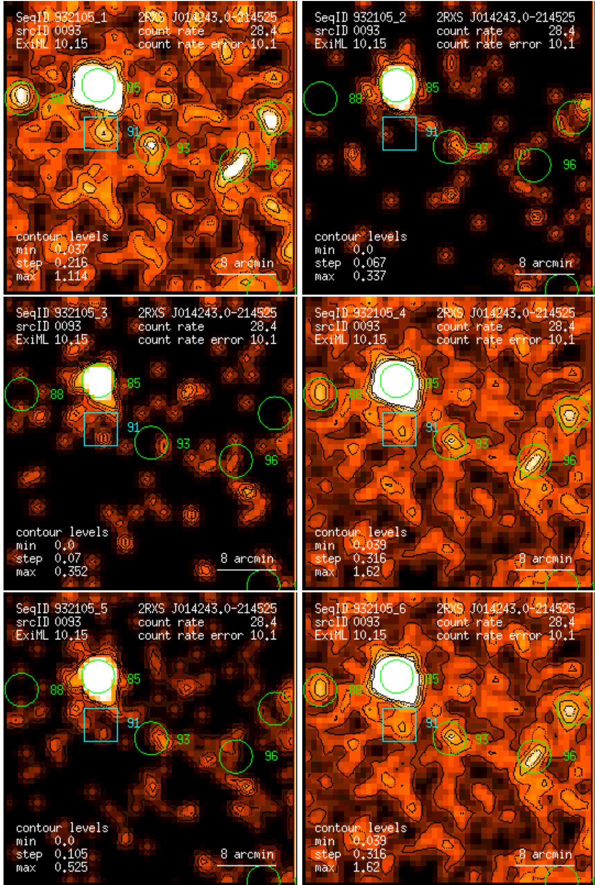
Figure 93: RASS 932105: detection 0093: band rate images, Gaussian filter: (1) PSPC channels 11 – 41, (2) 52 – 90, (3) 91 – 201, (4) 11 – 235, (5) 52 – 201, (6) 11 – 201. Broad band rates in counts/ks. Band rate contour levels in counts/ks/arcmin 2 .
