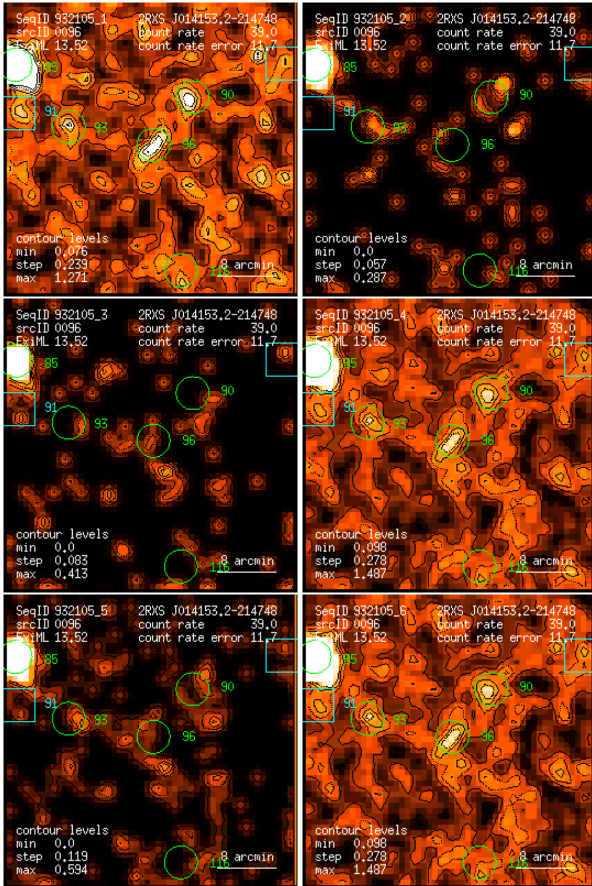
Figure 96: RASS 932105: detection 0096: band rate images, Gaussian filter: (1) PSPC channels 11 – 41, (2) 52 – 90, (3) 91 – 201, (4) 11 – 235, (5) 52 – 201, (6) 11 – 201. Broad band rates in counts/ks. Band rate contour levels in counts/ks/arcmin 2 .
