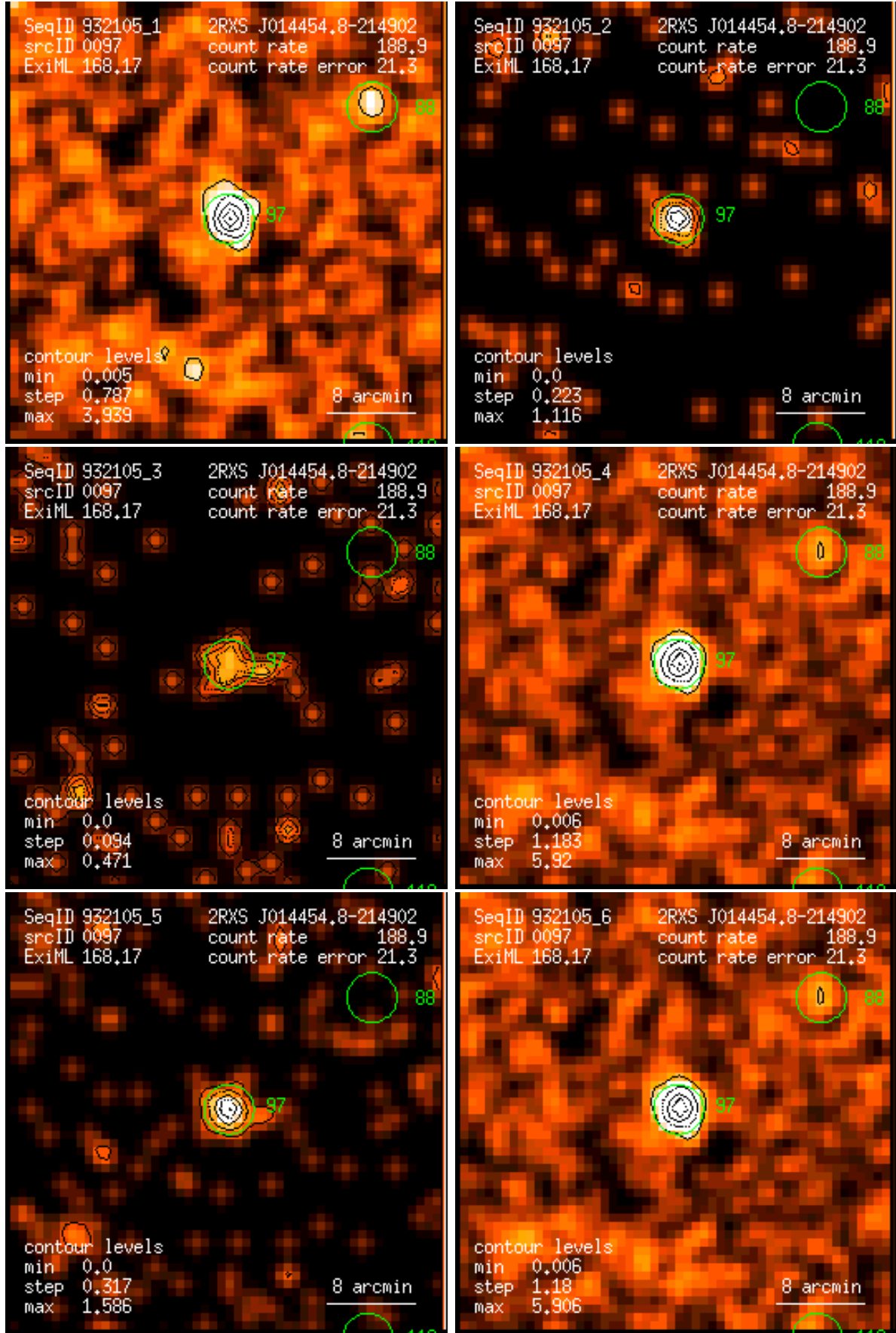
Figure 97: RASS 932105: detection 0097: band rate images, Gaussian filter: (1) PSPC channels 11 – 41, (2) 52 – 90, (3) 91 – 201, (4) 11 – 235, (5) 52 – 201, (6) 11 – 201. Broad band rates in counts/ks. Band rate contour levels in counts/ks/arcmin 2 .
