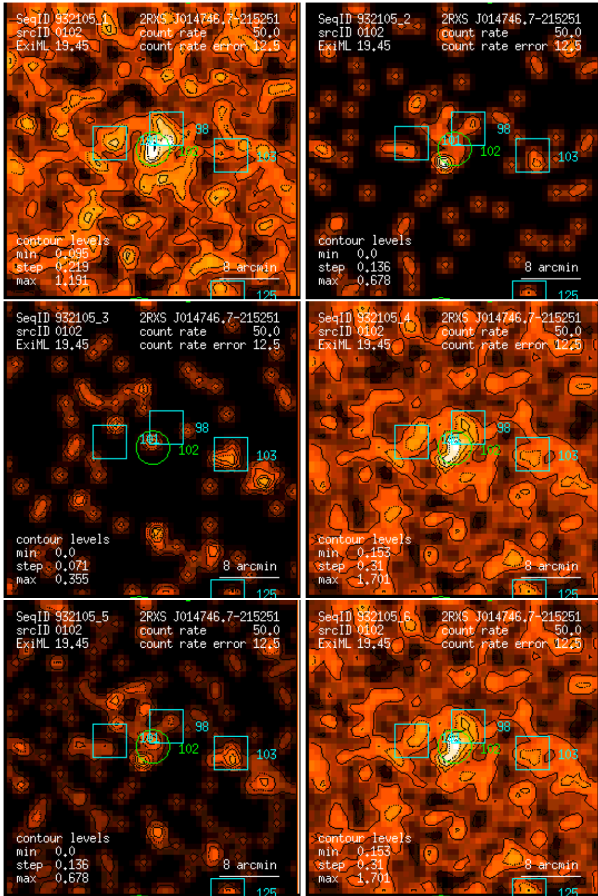
Figure 102: RASS 932105: detection 0102: band rate images, Gaussian filter: (1) PSPC channels 11 – 41, (2) 52 – 90, (3) 91 – 201, (4) 11 – 235, (5) 52 – 201, (6) 11 – 201. Broad band rates in counts/ks. Band rate contour levels in counts/ks/arcmin 2 .
