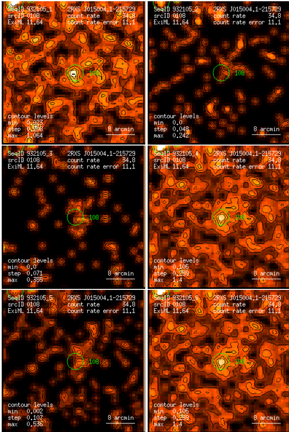
Figure 108: RASS 932105: detection 0108: band rate images, Gaussian filter: (1) PSPC channels 11 – 41, (2) 52 – 90, (3) 91 – 201, (4) 11 – 235, (5) 52 – 201, (6) 11 – 201. Broad band rates in counts/ks. Band rate contour levels in counts/ks/arcmin 2 .
