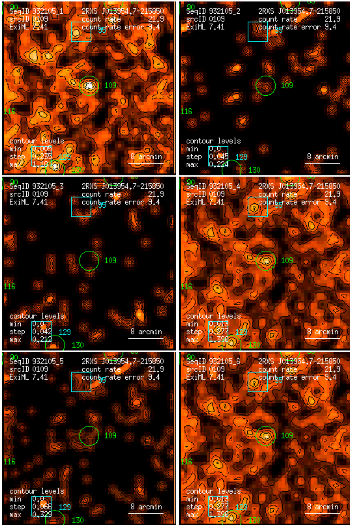
Figure 109: RASS 932105: detection 0109: band rate images, Gaussian filter: (1) PSPC channels 11 – 41, (2) 52 – 90, (3) 91 – 201, (4) 11 – 235, (5) 52 – 201, (6) 11 – 201. Broad band rates in counts/ks. Band rate contour levels in counts/ks/arcmin 2 .
