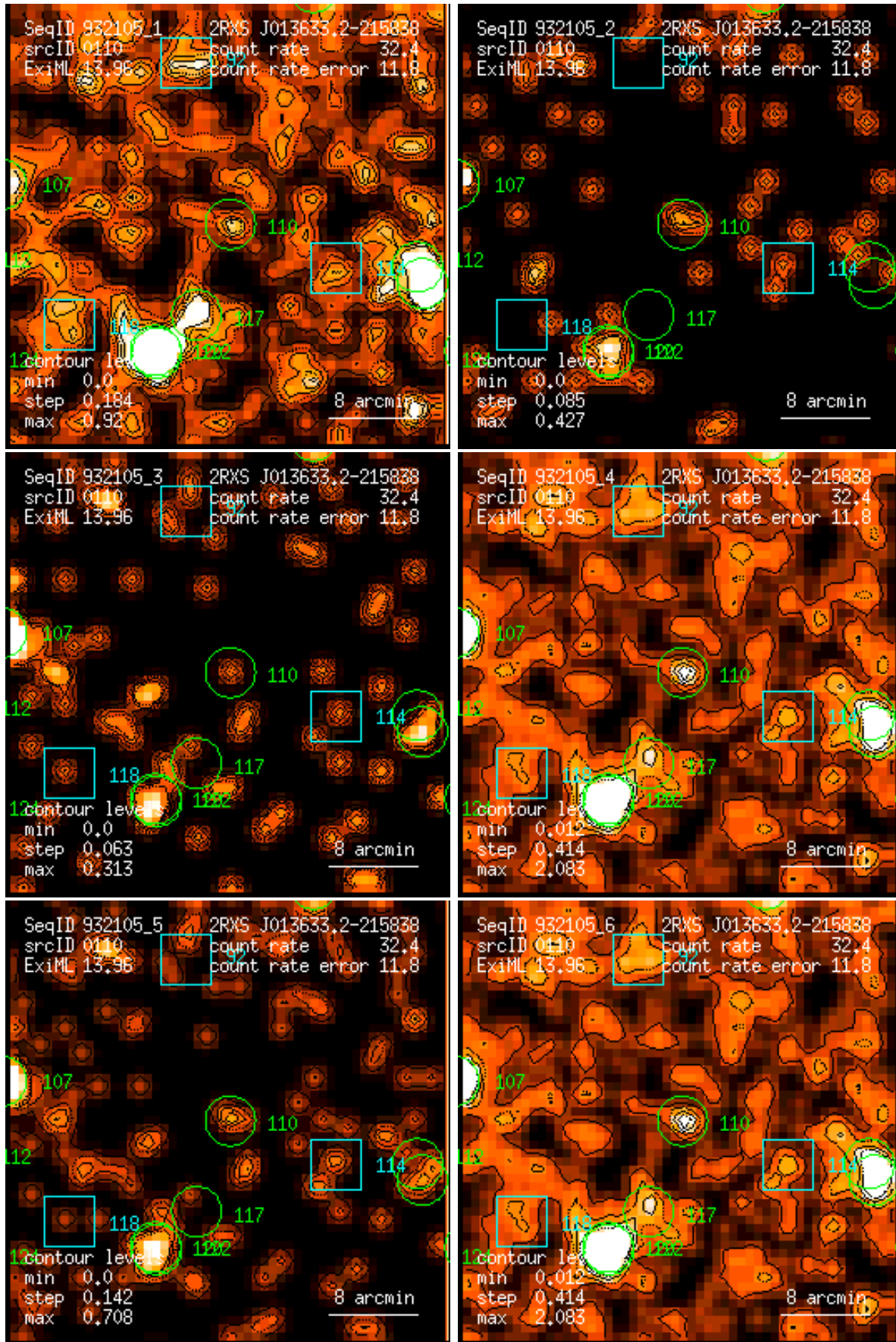
Figure 110: RASS 932105: detection 0110: band rate images, Gaussian filter: (1) PSPC channels 11 – 41, (2) 52 – 90, (3) 91 – 201, (4) 11 – 235, (5) 52 – 201, (6) 11 – 201. Broad band rates in counts/ks. Band rate contour levels in counts/ks/arcmin 2 .
