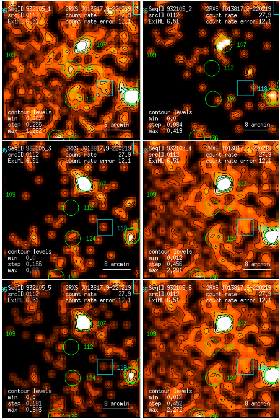
Figure 112: RASS 932105: detection 0112: band rate images, Gaussian filter: (1) PSPC channels 11 – 41, (2) 52 – 90, (3) 91 – 201, (4) 11 – 235, (5) 52 – 201, (6) 11 – 201. Broad band rates in counts/ks. Band rate contour levels in counts/ks/arcmin 2 .
