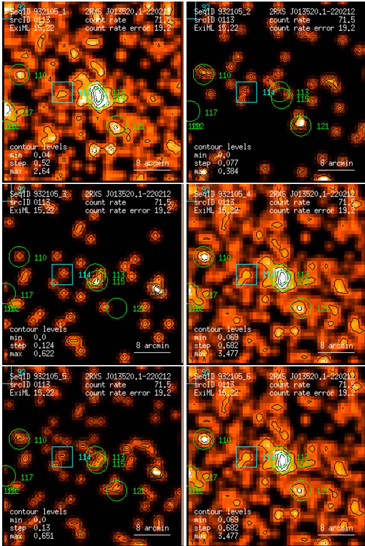
Figure 113: RASS 932105: detection 0113: band rate images, Gaussian filter: (1) PSPC channels 11 – 41, (2) 52 – 90, (3) 91 – 201, (4) 11 – 235, (5) 52 – 201, (6) 11 – 201. Broad band rates in counts/ks. Band rate contour levels in counts/ks/arcmin 2 .
