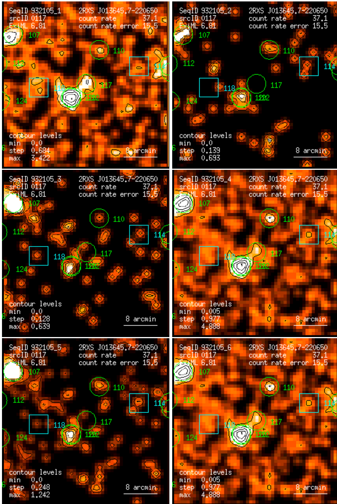
Figure 117: RASS 932105: detection 0117: band rate images, Gaussian filter: (1) PSPC channels 11 – 41, (2) 52 – 90, (3) 91 – 201, (4) 11 – 235, (5) 52 – 201, (6) 11 – 201. Broad band rates in counts/ks. Band rate contour levels in counts/ks/arcmin 2 .
