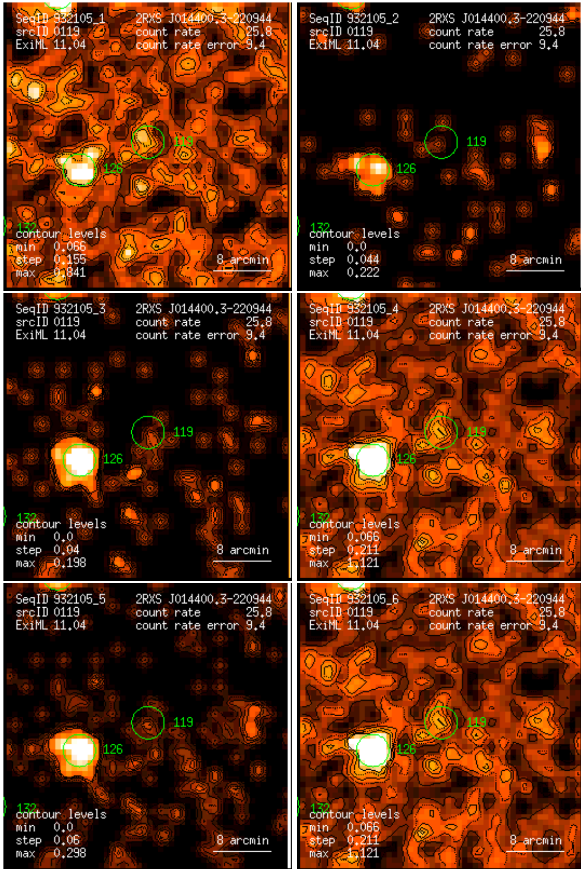
Figure 119: RASS 932105: detection 0119: band rate images, Gaussian filter: (1) PSPC channels 11 – 41, (2) 52 – 90, (3) 91 – 201, (4) 11 – 235, (5) 52 – 201, (6) 11 – 201. Broad band rates in counts/ks. Band rate contour levels in counts/ks/arcmin 2 .
