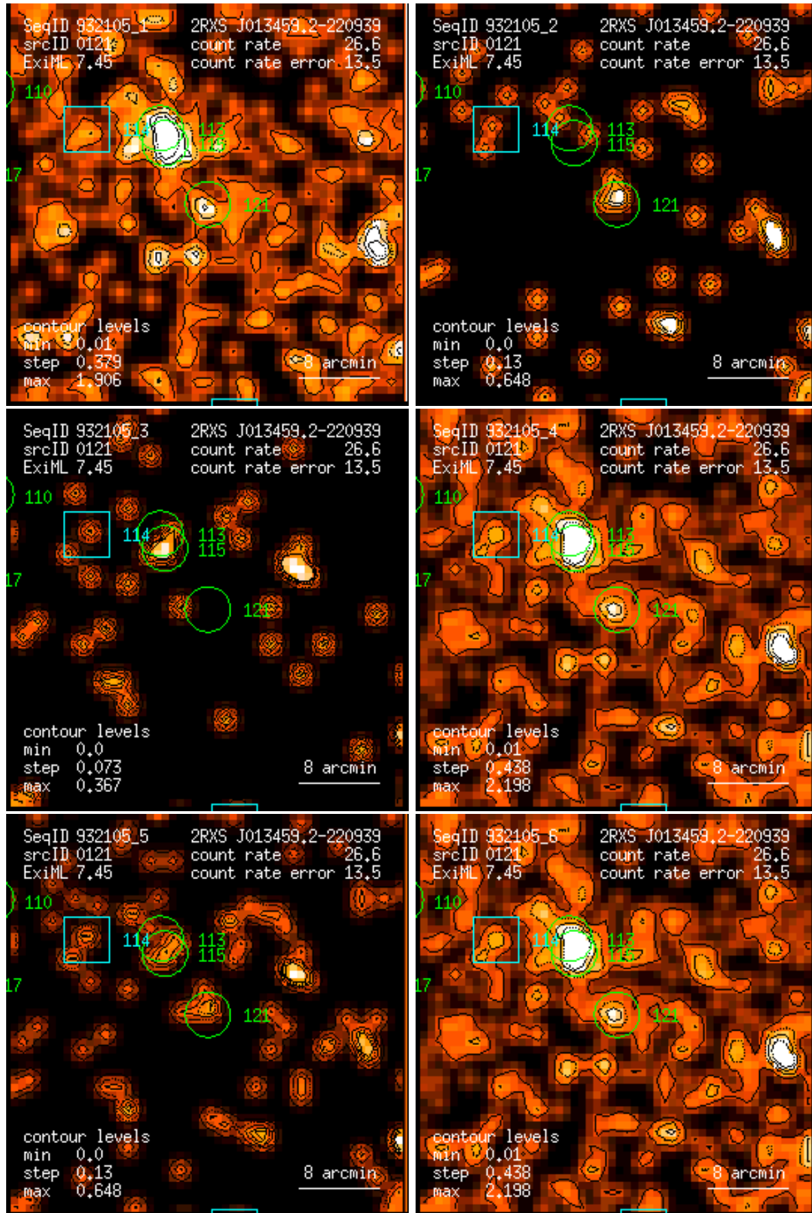
Figure 121: RASS 932105: detection 0121: band rate images, Gaussian filter: (1) PSPPC channels 11 – 41, (2) 52 – 90, (3) 91 – 201, (4) 11 – 235, (5) 52 – 201, (6) 11 – 201. Broad band rates in counts/ks. Band rate contour levels in counts/ks/arcmin 2 .
