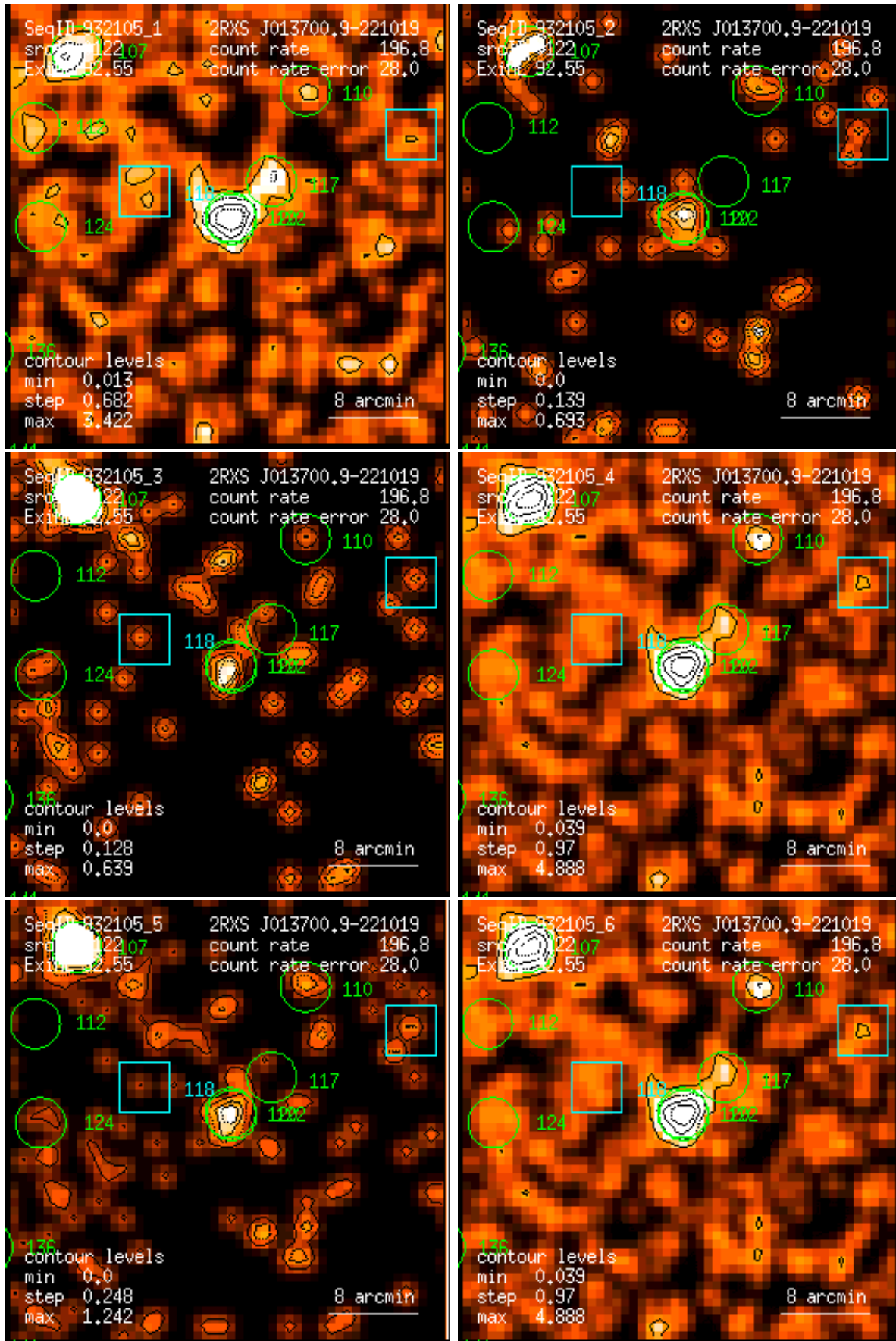
Figure 122: RASS 932105: detection 0122: band rate images, Gaussian filter: (1) PSPC channels 11 – 41, (2) 52 – 90, (3) 91 – 201, (4) 11 – 235, (5) 52 – 201, (6) 11 – 201. Broad band rates in counts/ks. Band rate contour levels in counts/ks/arcmin 2 .
