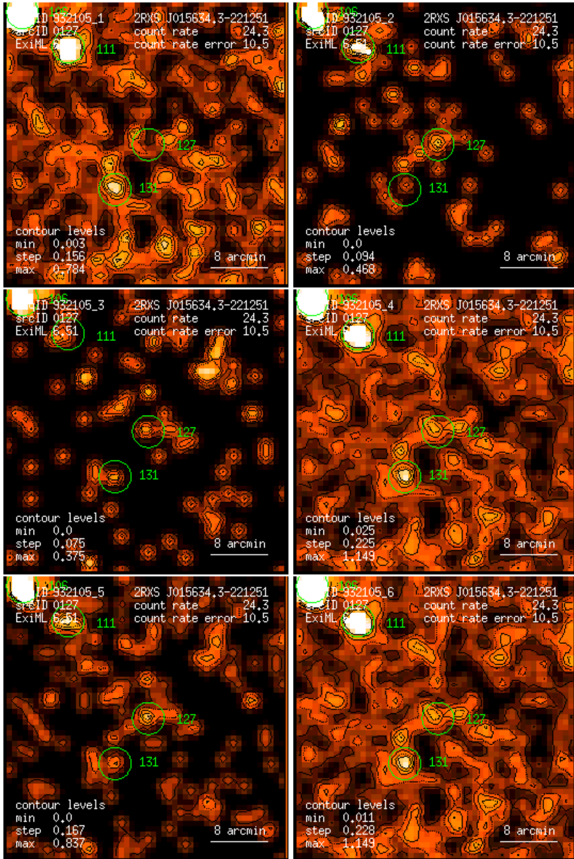
Figure 127: RASS 932105: detection 0127: band rate images, Gaussian filter: (1) PSPC channels 11 – 41, (2) 52 – 90, (3) 91 – 201, (4) 11 – 235, (5) 52 – 201, (6) 11 – 201. Broad band rates in counts/ks. Band rate contour levels in counts/ks/arcmin 2 .
