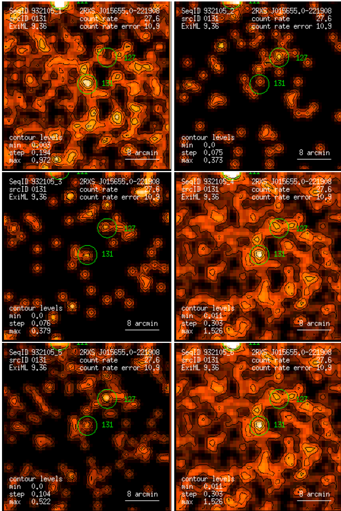
Figure 131: RASS 932105: detection 0131: band rate images, Gaussian filter: (1) PSPC channels 11 – 41, (2) 52 – 90, (3) 91 – 201, (4) 11 – 235, (5) 52 – 201, (6) 11 – 201. Broad band rates in counts/ks. Band rate contour levels in counts/ks/arcmin 2 .
