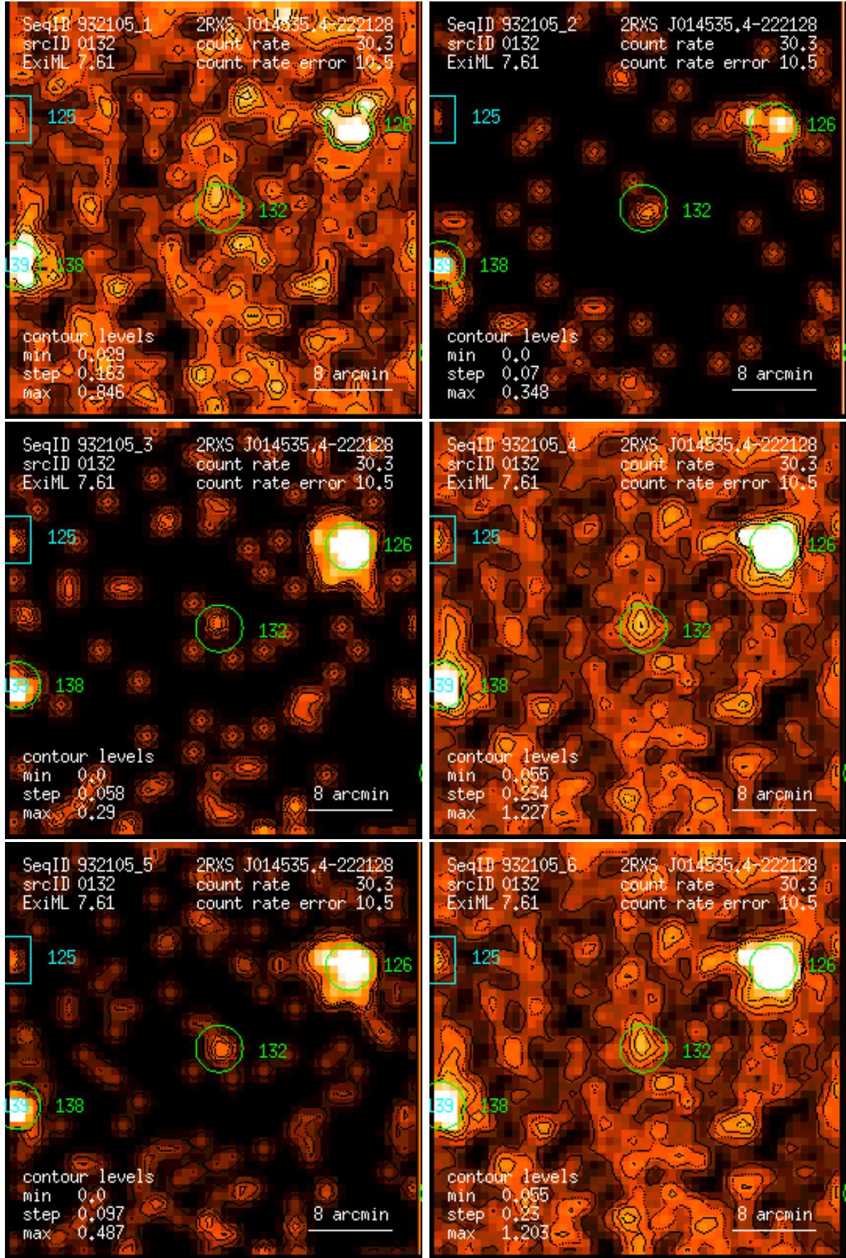
Figure 132: RASS 932105: detection 0132: band rate images, Gaussian filter: (1) PSPC channels 11 – 41, (2) 52 – 90, (3) 91 – 201, (4) 11 – 235, (5) 52 – 201, (6) 11 – 201. Broad band rates in counts/ks. Band rate contour levels in counts/ks/arcmin 2 .
